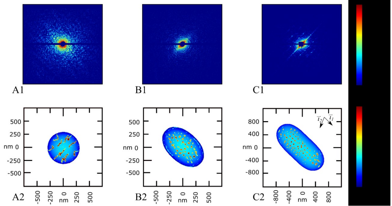
Figure 2. Diffraction patterns from Xe-doped droplets with various shapes: (A1) axisymmetric, nearly spherical, (B1) triaxial pseudo-ellipsoidal and (C1) capsule-shaped. The horizontal stripe in A1-C1 results from the gap between the upper and lower detector panels. Panels A2-C2 show column densities retrieved via the DCDI algorithm. The basis vectors of the vortex lattice in C2 are shown in the upper right corner of the panel.
