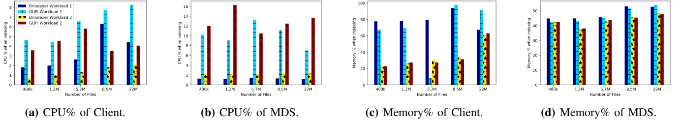
Fig. 8: Resource utilization during indexing by BRINDEXER and GUF1.
