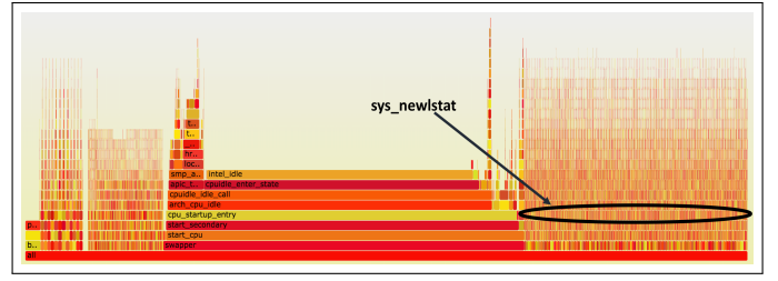
(b) Flame Graph for indexing with GUFFI.
