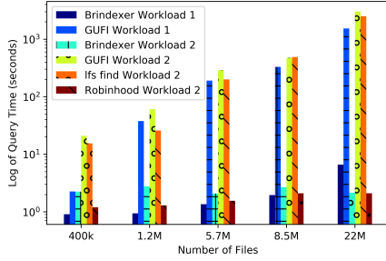
Fig. 9: Time taken to query by BRINDEXER, GUF1, lfs find , and Robinhood.
