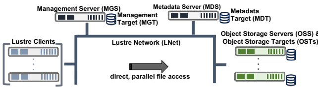
Fig. 2: An overview of Lustre architecture.
