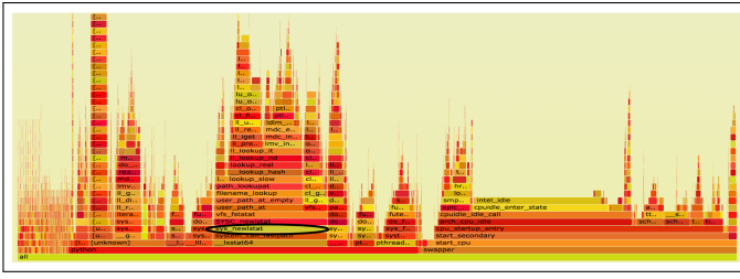
(a) Flame Graph for indexing with BRINDEXER.
