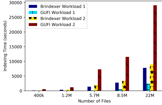
Fig. 7: Time taken to index by BRINDEXER and GUFFI.
