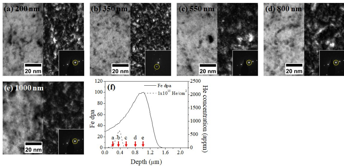
Figure 6. TEM bright-field and dark-field images of the 1 \times 10^{15} He preimplanted and Fe irradiated sample at depths of (a) 200, (b) 350, (c) 550, (d) 800, and (e) 1000 nm. Diffraction patterns obtained from the same grain are superimposed on each DF image with g110 marked by a yellow circle. (f) SRIM calculations of Fe, dpa, and He implant distributions are included, with red arrows indicating the depths of characterization. The dispersoid density was greatly increased in (b).
