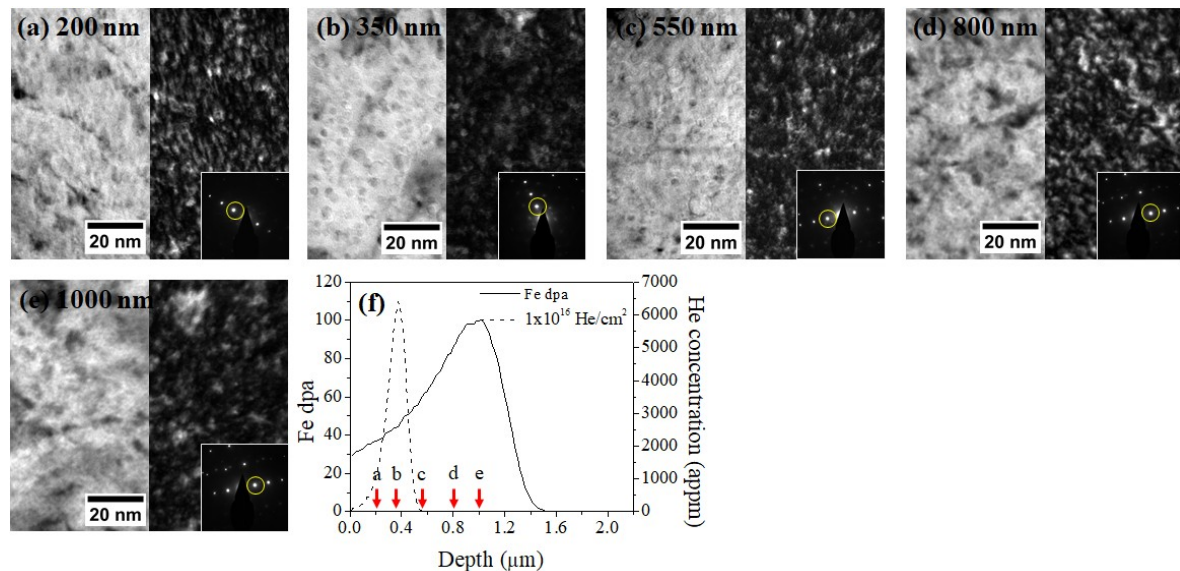
Figure 8. TEM bright-field and dark-field micrographs of the 1 \times 10^{16} He preimplanted and Fe irradiated specimen taken from depths of (a) 200, (b) 350, (c) 550, (d) 800, and (e) 1000 nm. Diffraction patterns obtained from the same grain are superimposed on each DF image with g110 marked by a yellow circle. (f) SRIM calculations are provided to show the depths of TEM characterization. A dispersoid density increase was not observed in (b).
