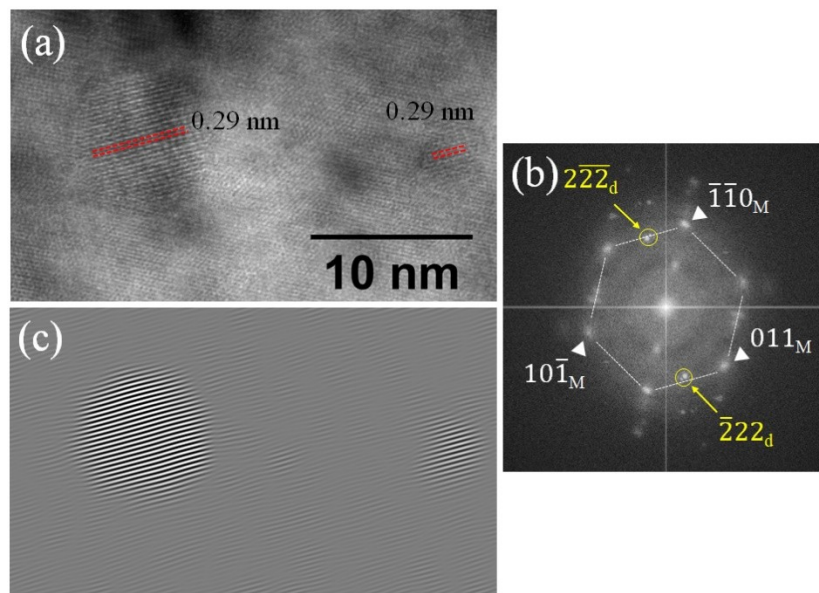
Figure 4. (a) High-resolution TEM (HRTEM) of two oxide dispersoids, (b) fast Fourier transform (FFT) patterns from the HRTEM, and (c) inverse FFT image of dispersoids using FFT patterns in yellow circles. The d -spacings measured from HRTEM and FFT patterns are 0.29 nm, which agree with (222) of pyrochlore Y_2Ti_2O_7 . The scale bar in (a) applies to (c).
