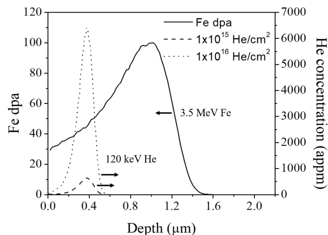
Figure 2. Stopping and Range of Ions in Matter (SRIM) calculations of damage profiles resulting from 3.5 MeV Fe ion irradiation and the He distributions resulting from 120 keV He ion implantation.
