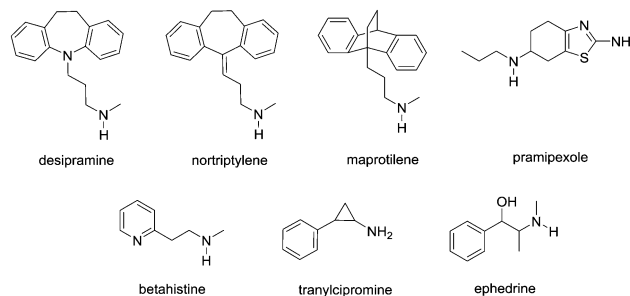
Fig. 2 Structures of the drugs evaluated in the present study.
