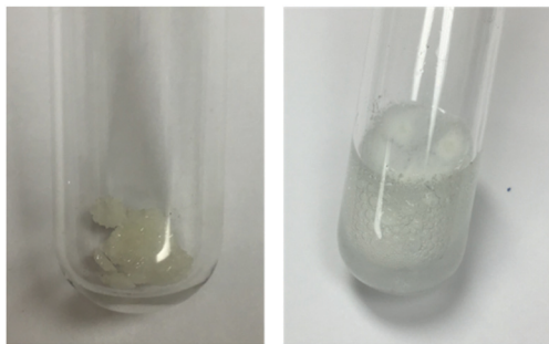
Fig. 3 Left: Crystals of the desipramine- \text{CO}_2 ammonium carbamate salt. Right: Same salt upon addition of water at pH = 2.0, within the normal gastric pH range. The evolution of \text{CO}_2 is apparent. Subsequent evaporation of water and analysis by ^1\text{H} - and ^{13}\text{C} -NMR revealed the re-formation of desipramine hydrochloride, the form of the drug currently in clinical use.
