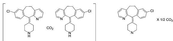
Fig. 1 Depictions of the proposed product of desloratadine combined with CO 2 , as duplicated from ref. 9a (left) and 9b (right). Note that while the depiction on the left reflects a composition (C 39 H 38 N 4 O 2 Cl 2 ) that matches the experimental elemental analysis (the depiction on the right does not), neither constitutes an unambiguous representation of a specific structure.
