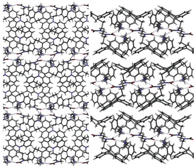
Fig. 5 Desipramine- \text{CO}_2 (left) and nortriptyline- \text{CO}_2 (right) crystalline products. Three layers shown; H-bonds indicated by green dashed lines. Desipramine- \text{CO}_2 : The layers have an all-hydrocarbon interior, save for the tertiary amine centres. H-bonding occurs on the layer surfaces between carbamate and amine groups; also, the gap between layers is spanned by H-bonds. Nortriptyline- \text{CO}_2 : The layer surfaces are nonpolar, populated by \pi faces of inclined phenyl groups of the carbamate species and by hydrogens of the amine species; each layer is made of distinct upper and lower sublayers joined at an interior seam where the ionic functional groups are located and H-bonding occurs.
