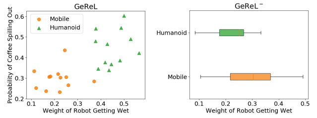
Figure 5: Feature weights learned by \text{GeReL} and \text{GeReL}^- .
