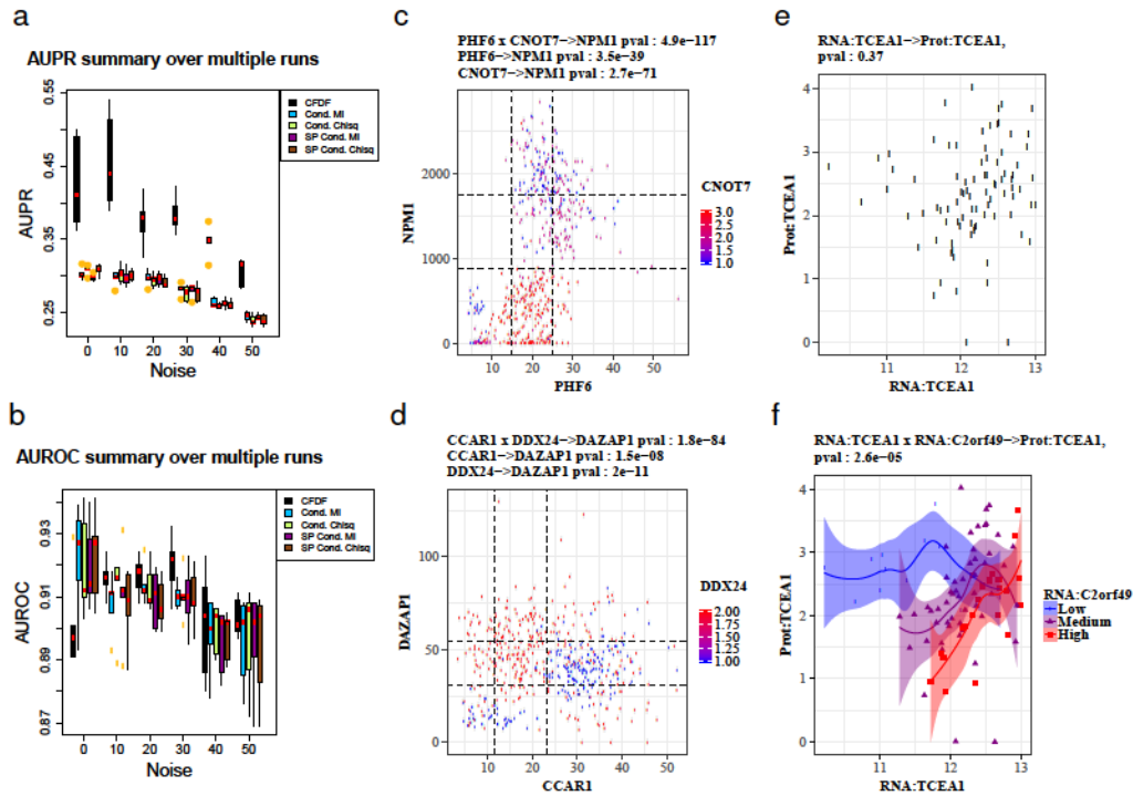
Figure 1: Result summary. (a) AUPR and (b) AUROC over multiple runs with increasing jitter noise. (c) PHF6 \times CNOT7 \rightarrow NPM1 and (d) CCAR1 \times DDX24 \rightarrow DAZAP1 , where the X-axis is the first parent, Y-axis the child, and color represents the second parent. The dotted lines represent the quantization levels. (e) and (f) C2orf49 , TCEA1 's mRNA and protein form a strong combinatorial relationship ( P=2.6 \times 10^{-5} ), rebutting central dogma violation.
