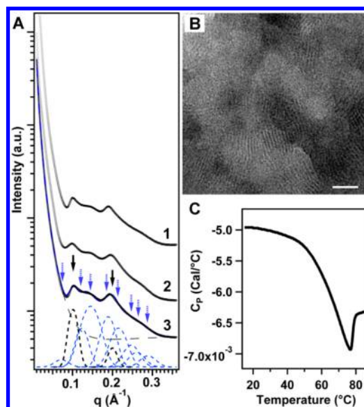
Figure 3. CIDR induces spontaneous PR reconstitution into “frozen” \text{PS-}b\text{-(P4MVP)}_2 membranes. (A) Synchrotron SAXS of proteopolymer complexes (trace 1: PR and \text{PS}_{26}\text{-}b\text{-(P4MVP)}_{21} ; trace 2: PR and \text{PS}_{38}\text{-}b\text{-(P4MVP)}_{21} ; trace 3: PR and \text{PS}_{42}\text{-}b\text{-(P4MVP)}_{29} ). The SAXS spectra are characterized by two strong harmonics (marked by black solid arrows) and a series of diffusive scatterings that are clearly discernible albeit weak (marked by blue dotted arrows). As an example shown for trace 3, the SAXS spectra are fitted to reveal a background scattering (dashed line), a multilamellar proteomembrane structure (black dotted peaks, q_{001} = 0.101 \text{ \AA}^{-1} ) that agrees well with TEM observation (panel B), and a 2-D hexagonally packed PR lattice in individual membranes (blue dotted peaks centered at 0.072, 0.124, 0.145, 0.189, 0.215, 0.247, and 0.26 \text{ \AA}^{-1} , corresponding to q_{10}, q_{11}, q_{20}, q_{12}, q_{30}, q_{22} , and q_{13} , respectively; note that the first peak at q_{10} is shadowed by strong scattering in the vicinity of the beam stop and appears weak). The summation (solid blue trace) of all scattering contributions overlaps nicely with the scattering data ( \circ ). (B) TEM of proteopolymer complexes (PR and \text{PS}_{42}\text{-}b\text{-(P4MVP)}_{29} , stained with 1% UAc) confirms the multilamellar proteopolymer membrane structure ( d \approx 6.0 nm). Scale bar: 50 nm. (C) DSC confirms that the polymersome membrane ( \text{PS}_{26}\text{-}b\text{-(P4MVP)}_{21} ) is “frozen” ( T_g = 66.3 °C) in solution.
