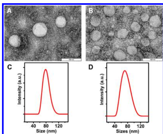
Figure 2. The amphiphilic triblock copolymers \text{PS-}b\text{-(P4MVP)}_2 self-assemble in water into polymersomes. The polymersome morphology of \text{PS}_{26}\text{-}b\text{-(P4MVP)}_{21} (A) and \text{PS}_{42}\text{-}b\text{-(P4MVP)}_{29} (B) is clearly revealed by TEM (scale bar: 100 nm; stained with 1% UAc), and their respective size distribution is confirmed by DLS (C, D).
