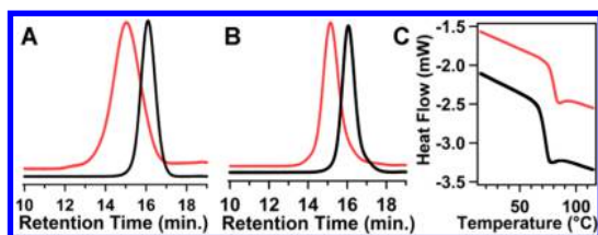
Figure 1. Well-defined amphiphilic triblock copolymers \text{PS-}b\text{-(P4MVP)}_2 prepared via controlled/living free radical polymerization methods. (A) GPC of \text{PS}_{26} block (black trace, M_n/\text{PDI} : 2600 Da/1.17) and \text{PS}_{26}\text{-}b\text{-(P4VP)}_{21} triblock copolymer (red trace, M_n/\text{PDI} : 7300 Da/1.22; shifted upward for clarity). (B) GPC of \text{PS}_{42} block (black trace, M_n/\text{PDI} : 4200 Da/1.18) and \text{PS}_{42}\text{-}b\text{-(P4VP)}_{29} triblock copolymer (red trace, M_n/\text{PDI} : 10 500 Da/1.10; shifted upward for clarity). (C) DSC of \text{PS}_{26} (black trace) and \text{PS}_{42} blocks (red trace) reveals their T_g at 71.3 and 79.6 °C, respectively.
