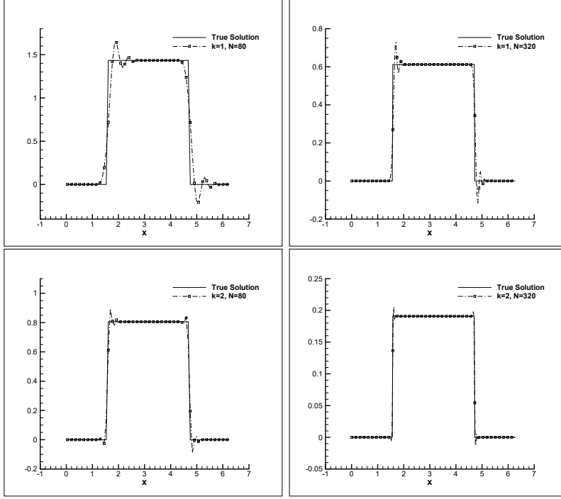
Fig. 4.1: Figures on (4.1) with M = 1 , b = 0.5 .
