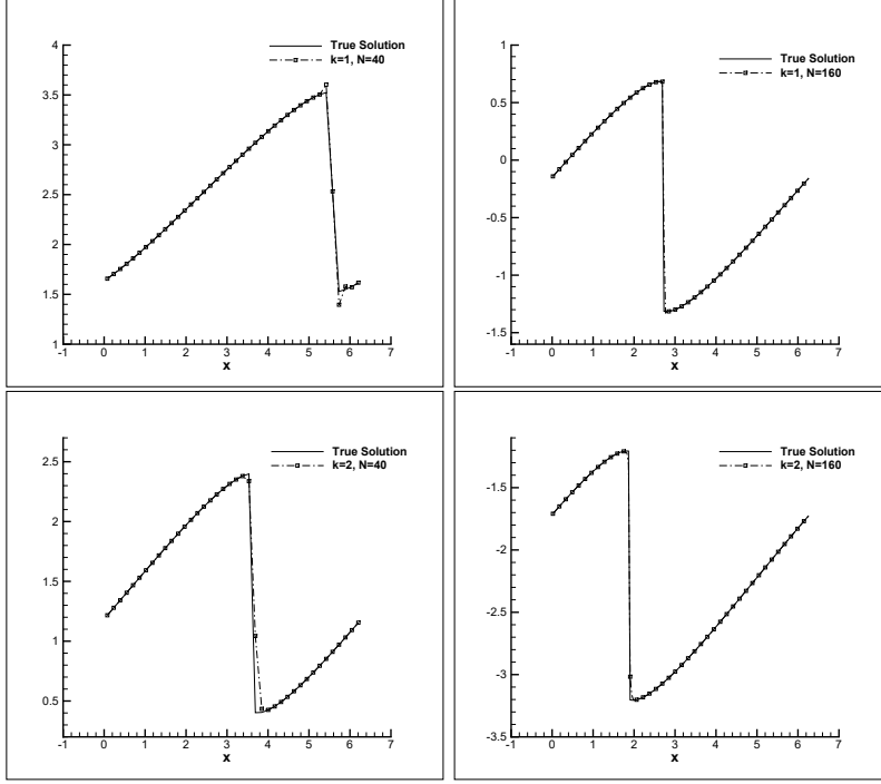
Fig. 4.2: Figures on (4.4) with M = 1 , b = 2.0 .
