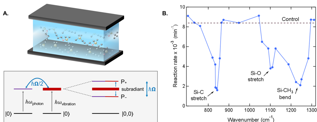
Figure 1. (A) The top panel shows a schematic of the microcavity enclosing a solution of the reagent. The bottom panel shows the bare single photon and single (collective) vibrational transitions and their corresponding vacuum state, |0\rangle . The coupling strength, \hbar\Omega/2 , is half of the so-called Rabi energy. In the VSC regime, new hybrid modes, separated by \hbar\Omega , are created (the upper ( P_+ ) and lower ( P_- ) VPs) at the expense of a large number of subradiant states remaining at the bare vibrational energy. The composite light-matter system ground state |0,0\rangle corresponds to the absence of any photon or vibrational excitations. (B) The overall reaction rate measured by Ebbesen, Moran, and co-workers as a function of the IR photon wavenumber. The out-of-cavity rate measured in a control experiment is shown as a dashed line. Clear reductions in rate are observed when the cavity is tuned to the vibrational transitions indicated in the figure.
