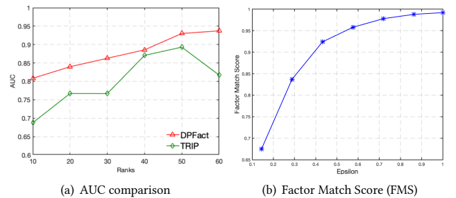
Figure 3: (a) Predictive performance (AUC) comparison for NICU between (1) TRIP, (2) DPFact. (b) Factor Match Score (FMS) under different privacy budget ( \epsilon ).
