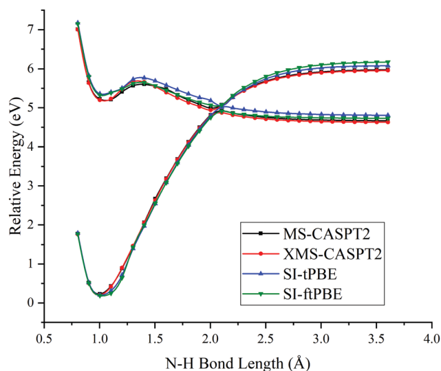
Fig. 3 PESs for N–H bond fission of eclipsed-H3 methylamine with various methods. The relative energies are compared with those of the equilibrium geometry for each method.
