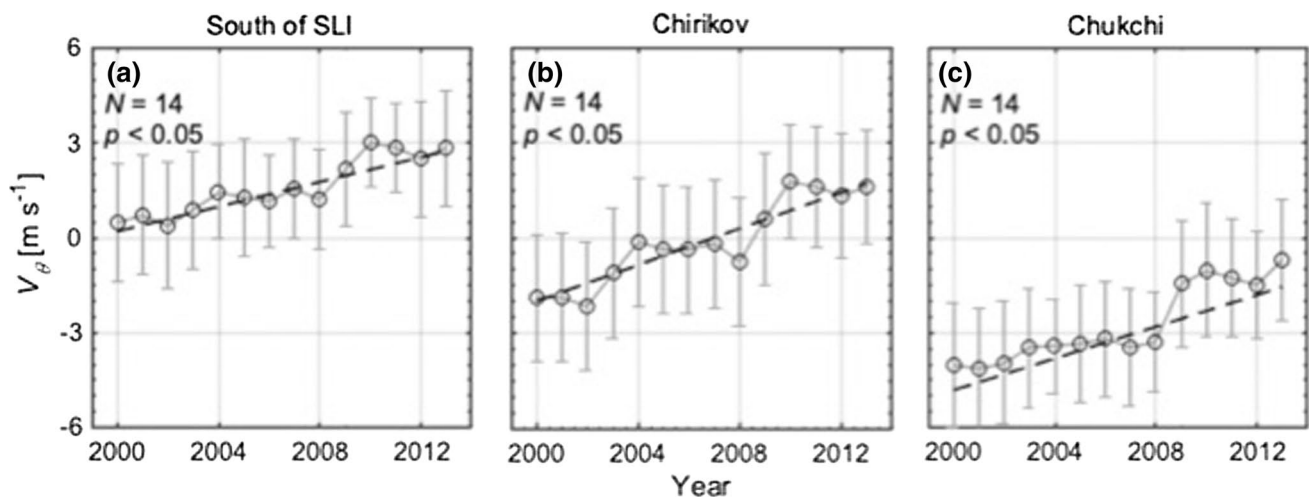
Fig. 5 Temporal trends in annual local wind velocities along best correlate directions ( V_\theta ) the benthic hotspots for 2000–2013 ( N=14 ). South of SLI, Chirikov, and Chukchi represent south of St. Lawrence Island (SLI), Chirikov Basin, and southeastern Chukchi Sea hotspots, respectively. \theta were 315^\circ , 330^\circ , and 0^\circ for south of SLI, Chirikov,
