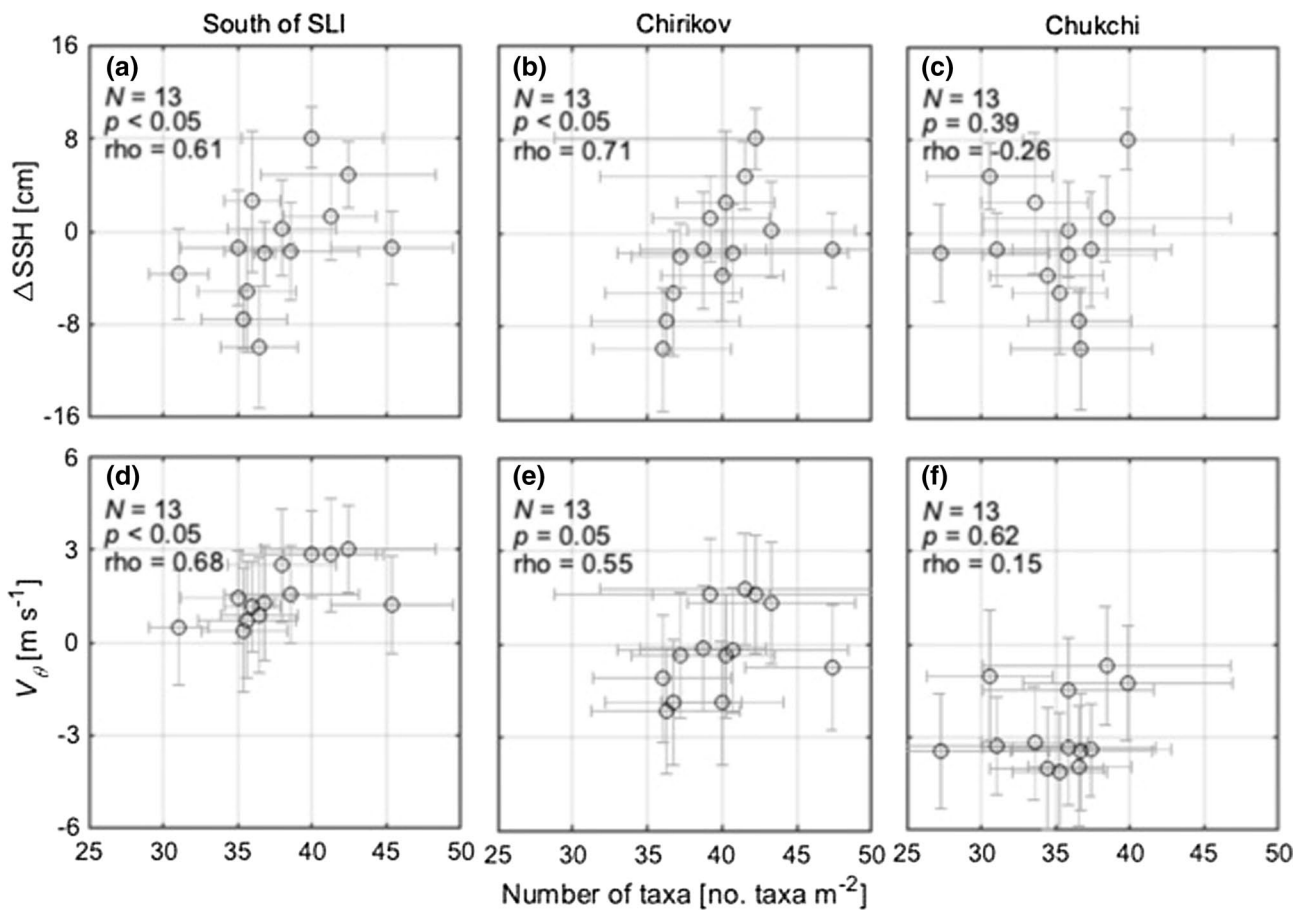
Fig. 7 Comparison results of number of taxa with difference in sea surface height between the Aleutian Basin and Chukchi Sea (ΔSSH) (a–c) and V_{\theta} (d–f) at the benthic hotspots during 2000–2013 ( N=13 ), respectively. South of SLI, Chirikov, and Chukchi represent south of
