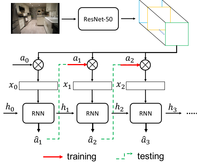
Figure 5: The general pipeline of the RNN-based methods. A pre-trained ResNet-50 is used to obtain the feature maps from an image, and at each step i we extract the feature vector \mathbf{x}_i at the human ground-truth fixation location a_i . This is done both during training (shown by solid red arrows) and during testing for fixation location prediction \hat{a}_i (shown by dashed green arrows). \mathbf{x}_i and \mathbf{h}_i are then fed into the RNN to predict the next fixation.
