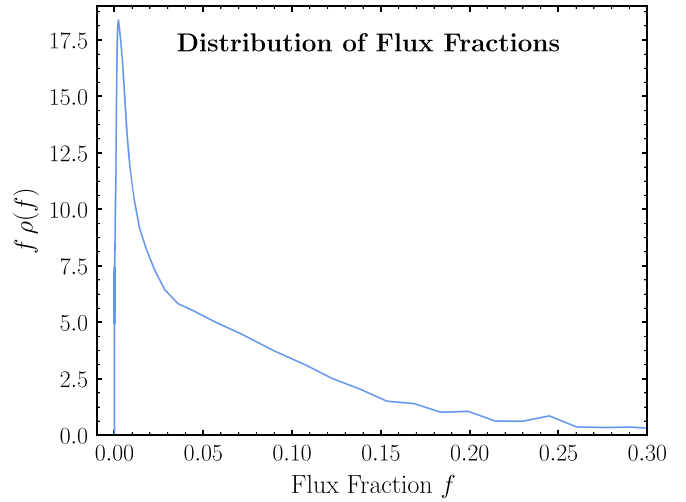
Figure 1. Distribution of the frequency of pixels that contain a fraction f of the flux from a point source, \rho(f) , for the full sky template, which is appropriate for modeling isotropic extragalactic sources. This quantity is central to incorporating the PSF of IceCube into the NPTF likelihood, according to Equation (16). We have chosen to show f\rho(f) , as following Equation (15) this quantity integrates to one given conservation of flux. See the text for details.
