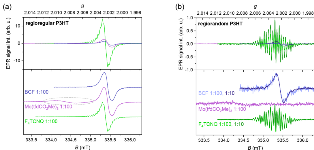
Figure 4. X-band room temperature cw EPR spectra recorded on solutions of rreP3HT (a) and rraP3HT (b) doped with F 4 TCNQ, BCF or Mo(tfd-CO 2 Me) 3 in chloroform at doping ratios of 1:100 (and 1:10 for rraP3HT). The signal intensities normalized by Q-factor and modulation amplitude are compared in the top part of the graphs and the normalized spectra are shown in the bottom part for comparison of the spectral shapes. The signal from the Mo(tfd-CO 2 Me) 3 anion is highlighted by the dashed grey line. The spectra are shown for a microwave frequency of 9.4 GHz, additional experimental details are described in the Experimental Methods section and the SI.
