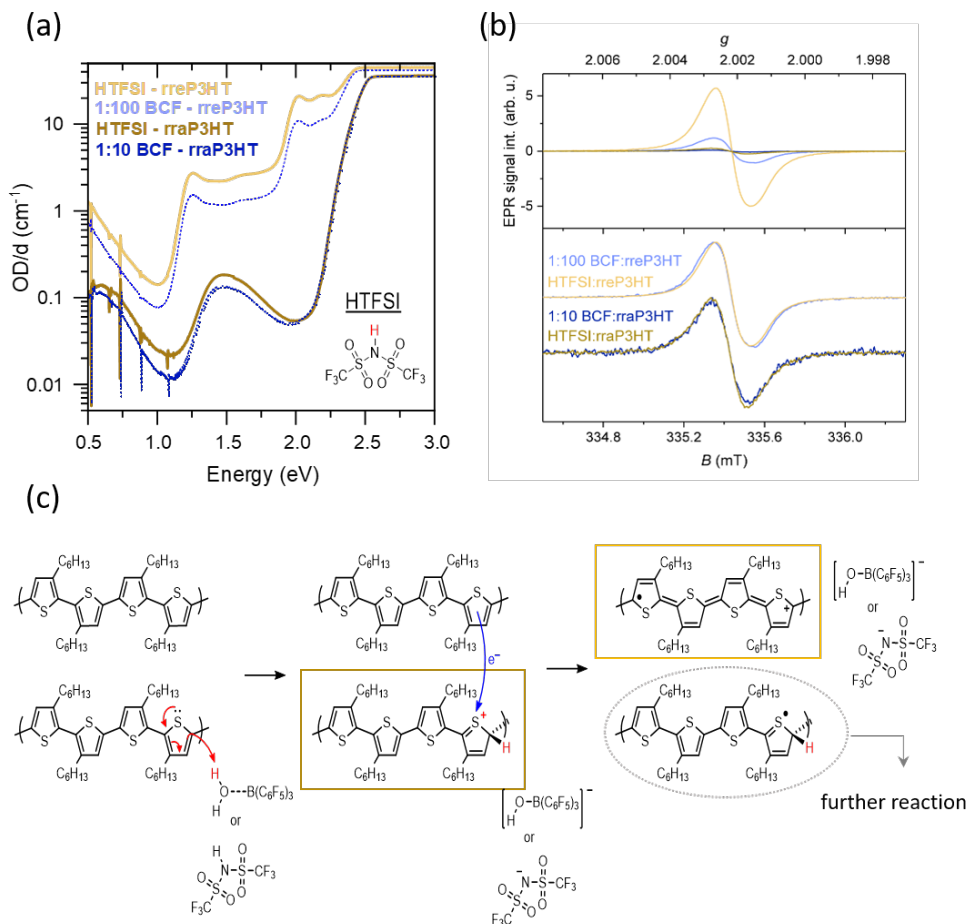
Figure 5. (a) Comparison of UV-Vis-NIR absorption spectra of rre- and rraP3HT solutions (in chloroform) doped with BCF and HTFSI (Inset: chemical structure of HTFSI) (b) Comparison of X-band room temperature cw EPR spectra recorded on solutions of rreP3HT and rraP3HT doped with BCF or HTFSI. The signal intensities normalized by Q-factor and modulation amplitude are compared in the top part of the graphs and the normalized spectra are shown in the bottom part for comparison of the spectral shapes. See the Experimental Methods section and the SI for additional experimental details. (c) Possible reaction mechanism between P3HT units and BCF or HTFSI following references 38, 65 , wherein the chain is first protonated (brown), leading to the creation of a spin-less protonated polymer cation and a negatively charged BCF:OH - complex. The subsequent electron transfer from a neutral chain or segment results in a P3HT radical cation (orange) and a neutral protonated radical (grey).
