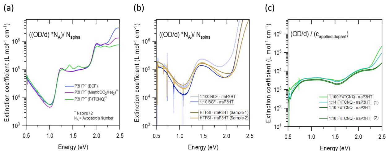
Figure 6. The molar extinction coefficient of a polaron on a) rreP3HT and b) rraP3HT, determined using the concentration of spins of charged P3HT (see Table S2) obtained from EPR spectroscopy. Shown in c) is the molar extinction spectrum of the CTC formed between F 4 TCNQ and rraP3HT, calculated from the optical absorption of different data sets with the presumption that every dopant forms one complex. Note that
