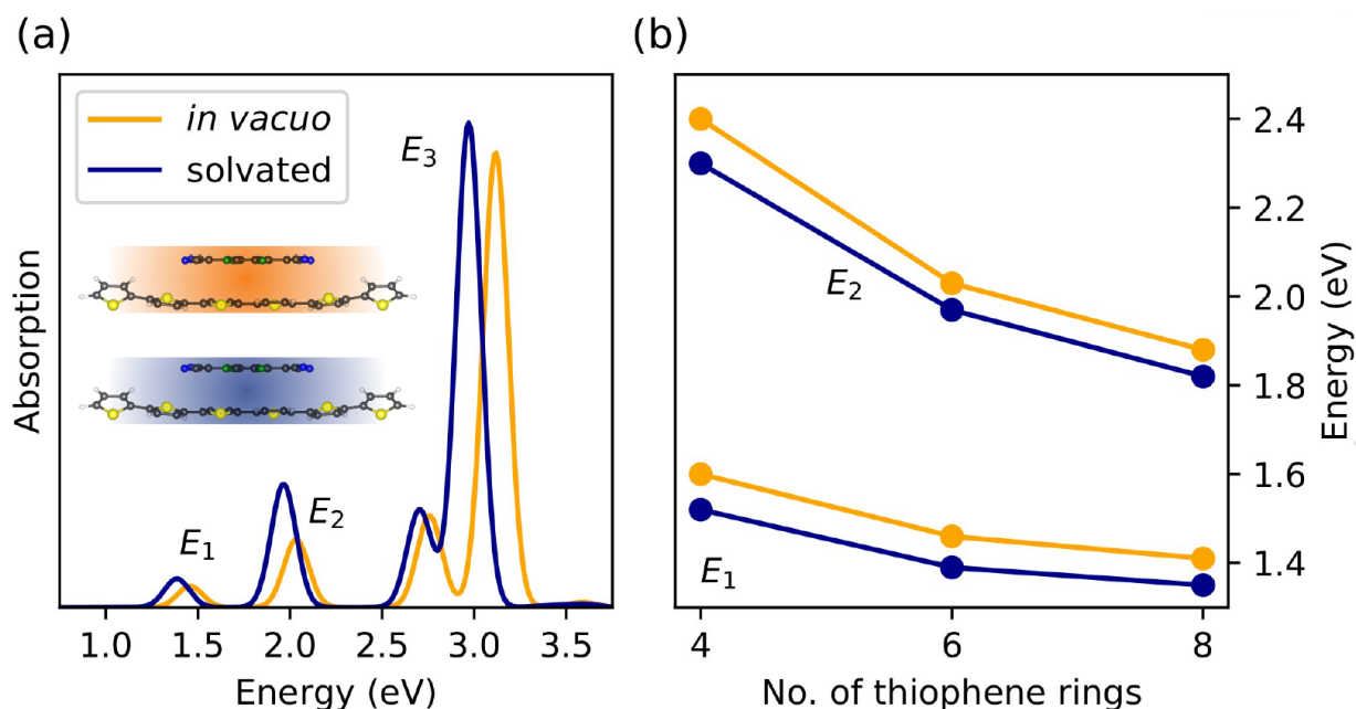
Figure 3. (a) Optical absorption spectra from TDDFT of the 6T:F4TCNQ bimolecular complex in vacuo (orange) and in chloroform (blue). The insets show the respective optimized geometries. (b) Energy of the absorption peaks E_1 and E_2 as a function of the length of the doped oligothiophene, in vacuo (orange) and in chloroform (blue). A Lorentzian broadening of 80 meV is applied to all spectra.
