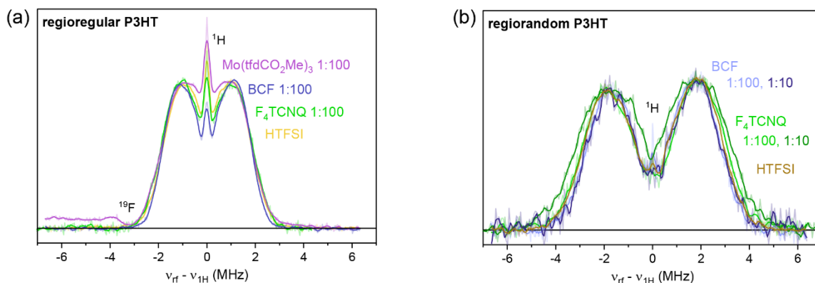
Figure 7. Q-band ^1\text{H} Davies ENDOR spectra recorded on frozen chloroform solutions of rreP3HT (a) and rraP3HT (b) doped with \text{F}_4\text{TCNQ} , BCF, HTFSI or \text{Mo}(\text{tfd-CO}_2\text{Me})_3 at doping ratios of 1:100 (and 1:10 for rraP3HT) at a temperature of 10 K. The ENDOR spectra were recorded at the maximum of the EPR signal of the P3HT radical cation, at a magnetic field around 1213.5 mT (see SI section 6 for further experimental details). The lower signal-to-noise ratio for the spectra in b) is due to the significantly smaller number of spin-carrying moieties in doped rraP3HT solutions.
