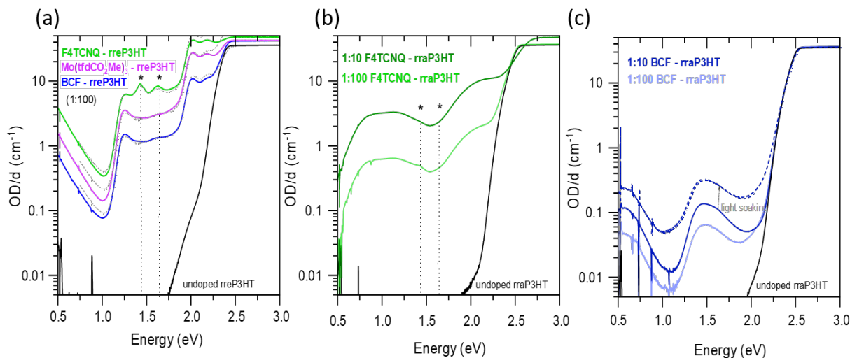
Figure 2. UV-Vis-NIR absorption spectra of solutions (in chloroform) of a) rreP3HT doped with F 4 TCNQ, Mo(tfd-CO 2 Me) 3 and BCF in the ratio 1:100 (dopant : repeat unit), b) rraP3HT with F 4 TCNQ (1:100 and 1:10) and c) rraP3HT with BCF (1:100, 1:10, light-soaked 1:10). The dashed grey lines in (a) correspond to the spectra reconstructed using the Beer-Lambert law, with a weighted fraction of the P3HT radical cation (polaron) spectrum (and the F 4 TCNQ radical anion spectrum in F 4 TCNQ-doped solution). The positions of the characteristic double peaks of the F 4 TCNQ radical anion are highlighted (*) for reference. Additional details are provided in the SI.
