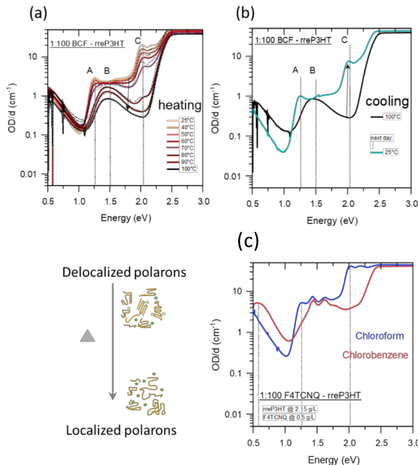
Figure 8. (a) Temperature-dependent UV-Vis-NIR solution spectra of 1:100 BCF-doped rreP3HT in chlorobenzene and (b) normalized spectra at 25°C and 100°C. The dash-dot lines show characteristic peak positions of the delocalized polaron (A), the localized polaron (B) and the P3HT aggregate peak (C). (selected spectra are also shown and discussed in ref 19 ) (c) Comparison of the UV-Vis-NIR absorption spectra of 1:100 F 4 TCNQ-doped rreP3HT solution in chloroform (blue) vs. chlorobenzene (red).
