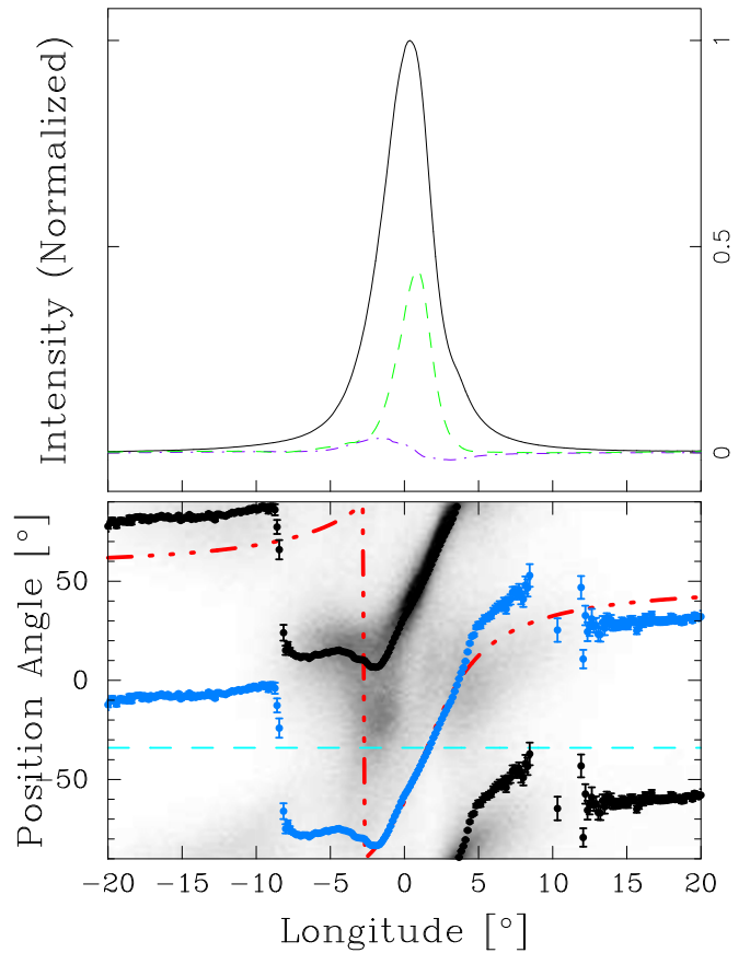
Figure 5. High-resolution MJD 58509 MP profile. The upper panel shows the average profile around the MP region, while the lower panel shows the single-pulse PPA distribution and average (black) along with the orthogonal PPA track (blue). The RVM curves and PM direction are shown as in Figure 1.
