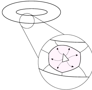
Figure 6. The restriction of the triangulation to each of the B_i ( i \in S ), up to taking two barycentric subdivisions, is shellable. By counting the number of ways in which two of the B_i 's can be glued to one another, we determine an upper bound on the number of triangulations.
