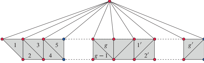
Figure 4. To construct g! triangulations of the genus- g surface, fix a bijection \pi: \{1, \dots, g\} \rightarrow \{1, \dots, g'\} . Take a strip of 2g + 3 triangles as above, and cone off its boundary to get a 2-sphere with 4g + 5 triangles. Now remove the interiors of the 2g triangles 1, \dots, g, 1', \dots, g' , and create a genus- g surface by attaching handles between the hole i and the hole \pi(i) , for all i . Since every handle can be triangulated using 12 triangles, this yields a triangulation T_\pi with 14g + 5 triangles of the genus- g surface. By inspecting the link of the highest-degree vertex, from T_\pi we can recover \pi , which implies that different permutations yield different triangulations.
