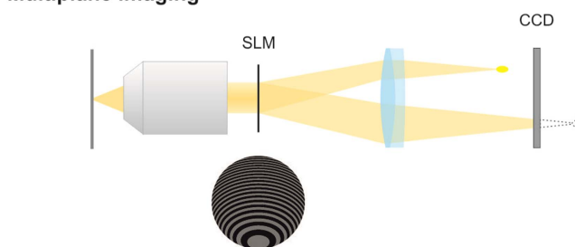
Figure 14. Examples of microscopy methods structuring light on the detection side: Fourier filtering, multiplexing.
