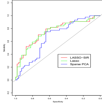
FIG 1. ROC curve of various methods for Arcene Data set.
