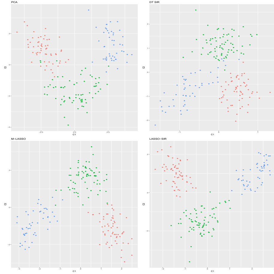
FIG 2. We plotted the second component versus the first component for all the wines, which are labeled with different colors, representing different cultivars (1-red, 2-green, 3-blue). The four methods for calculating the directions are PCA, DT-SIR, M-Lasso, and Lasso-SIR from top-left to bottom-right. It is clearly seen that Lasso-SIR offered the best separation among these three groups.
