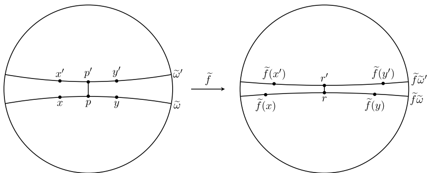
Figure 6. Bounding v_t from above.
