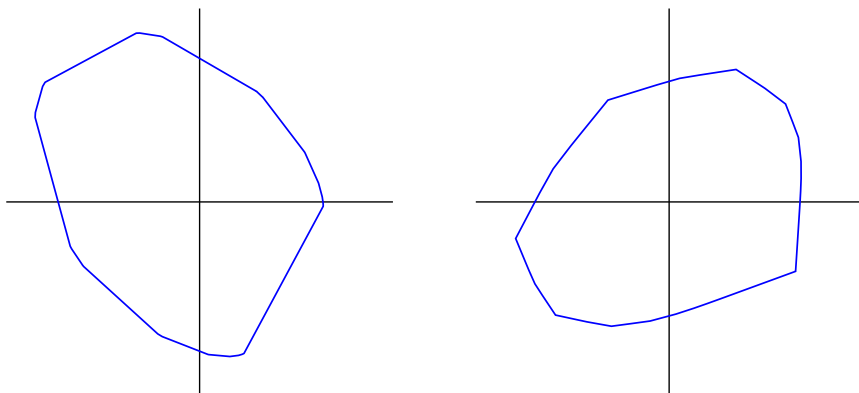
Figure 11. At left, the unit sphere T_X^1\mathcal{T}(S_{1,1}) of the Thurston norm on the tangent space at the point X = 0.35 + 1.8i in the upper half-plane model of \mathcal{T}(S_{1,1}) . At right, the unit sphere of the dual norm on the cotangent space.
