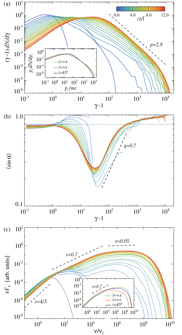
Figure 2. Time evolution of the particle spectrum (top panel), mean pitch angle (middle panel), and angle-integrated synchrotron spectrum (bottom panel) for the simulation in Figure 1. The insets of the top and bottom panels show, respectively, the particle momentum spectra and the synchrotron spectra at late times ( ct/l = 11 ) along +\hat{x} (green line), +\hat{z} (orange line), and at 45 degrees between +\hat{x} and +\hat{z} (blue line).
