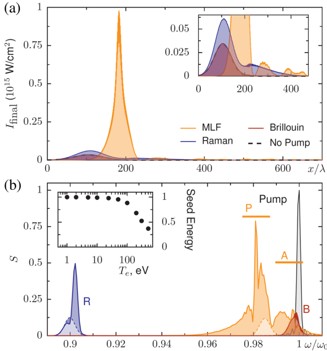
FIG. 4. PIC simulations of amplification via stimulated Raman (R), Brillouin (B), and MLF (P, A) scattering. (a) Seed after interaction in plasma ( N = 0.01 , L = 175\lambda ) with a counterpropagating pump ( a_0 = 0.007 , \lambda = 1 \mu\text{m} , I = 6.7 \times 10^{13} \text{ W/cm}^2 ). (b) Spectra of the initial (dashed) and amplified (solid) seed pulses for each mechanism, together with the pump. \lambda/\Delta x = 150 , 200 particles/cell, T_e = T_i = 1 eV and m_i/m_e = 1836 . For MLF, B_0 = 9900 T and \theta = 80^\circ . The initial seed intensities are half the pump intensity. Inset: variation in normalized seed final energy with T_e for MLF mechanism.
