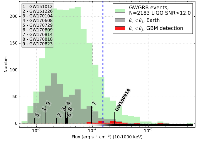
Figure 3. Expected gamma-ray flux distribution from BBH, arising from the Blandford Znajek mechanism (Section 3.2). The BBH-to-GRB ratio is 2183/24 = 91.0. The notations are similar to those of Figure 2.
