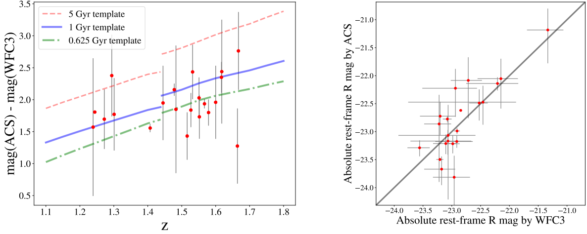
FIG. 5.— Left : The observed color as a function of redshift, based on 21/32 AGNs which have both WFC3 and ACS imaging data. Note that the filter combinations WFC3/F125W and WFC3/F140W are adopted for galaxies at z < 1.44 and z > 1.44 , respectively. We also plot three predicted models including 5 Gyr, 1 Gyr and 0.625 Gyr. Clearly, the 5 Gyr stellar population is ruled out by our data, and we adopt the 1 Gyr and 0.625 Gyr for galaxies at z < 1.44 and z > 1.44 , respectively. Right : Comparison of the inferred rest-frame R band magnitude, based on the adopted stellar populations.
