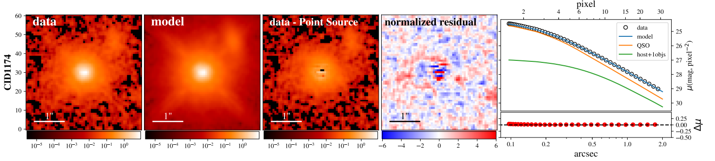
FIG. 2.— AGN-host galaxy decomposition of COSMOS-CID1174 based on the HST /WFC3 F140W image. The panels from left to right are as follows: (1) observed data, (2) best-fit model (AGN+host), (3) data minus the model PSF (i.e., host galaxy free of the AGN), (4) residuals divided by the variance and (5) 1-D surface brightness profiles (top) and the corresponding residual (bottom). The 1-D profiles indicate the surface brightness including the data (open circles), the best-fit model (blue line), the AGN (orange line), and the model for the extended sources (green line, i.e., host and other objects). Note that the 1-D surface brightness profiles are only for illustration purposes. The actual fitting is based on the two-dimensional images. The remaining 31 objects in the sample are shown in Appendix A.
