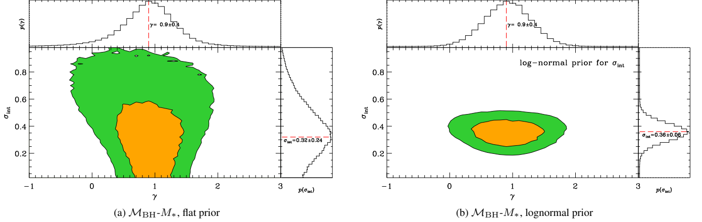
FIG. 10.— Constraining the evolution factor \gamma of \mathcal{M}_{\text{BH}}-M_* relation (Equation 9), with intrinsic scatter \sigma_{\text{int}} , using a Monte Carlo simulation. The adopted sample includes our 32 AGNs and the intermediate redshift AGNs, using flat prior of \sigma_{\text{int}} (left panel) and lognormal prior (right panel). The colored regions indicate the 68 and 95% confidence regions.
