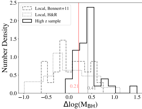
FIG. 9.— Histogram of the \log(\mathcal{M}_{\text{BH}}) offset for the local samples and our 32 high- z sample. The gray vertical line shows the mean value of the offset for the high- z sample, and the red vertical line shows the shift the expectation by the selection effect, even if there were no evolution. The median value of the offset is very close to the mean value (+0.30).
