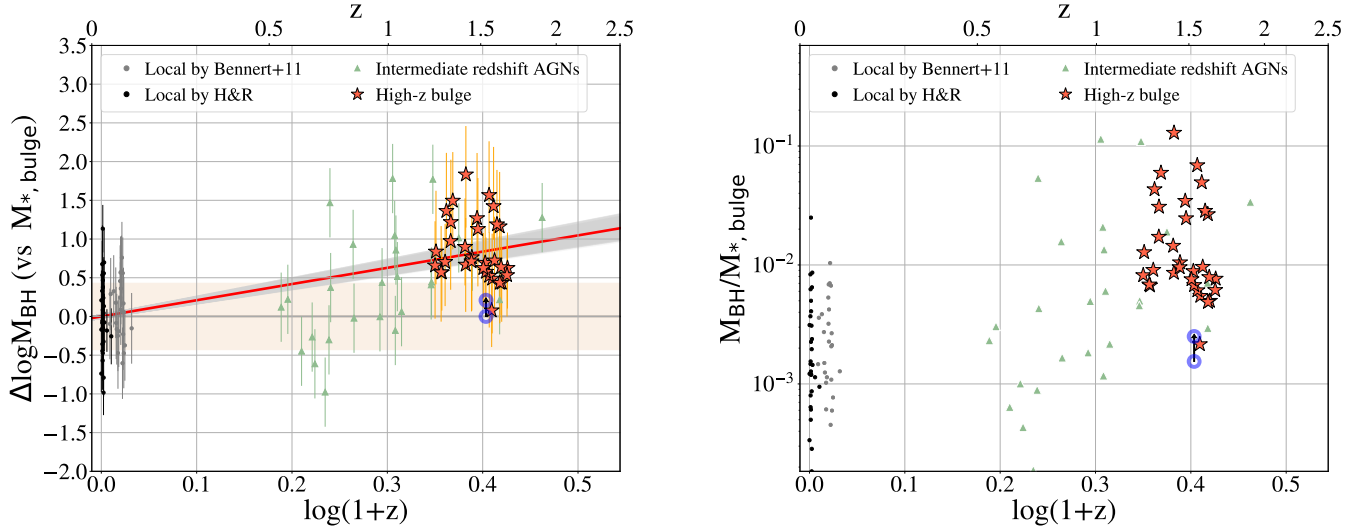
FIG. 13.— Same as Figure 8, but for \mathcal{M}_{\text{BH}}-M_{*,\text{bulge}} relations. The intermediate sample consists of 27 objects from Bennert et al. (2011b) and Schramm & Silverman (2013) , listed in Table 7. Cisternas et al. (2011) do not provide information to infer their bulge mass.
