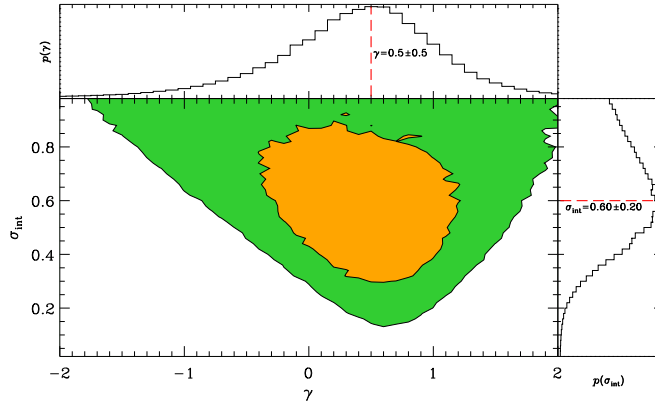
(c) \mathcal{M}_{\text{BH}}\text{-}L_{\text{host}} , flat prior
