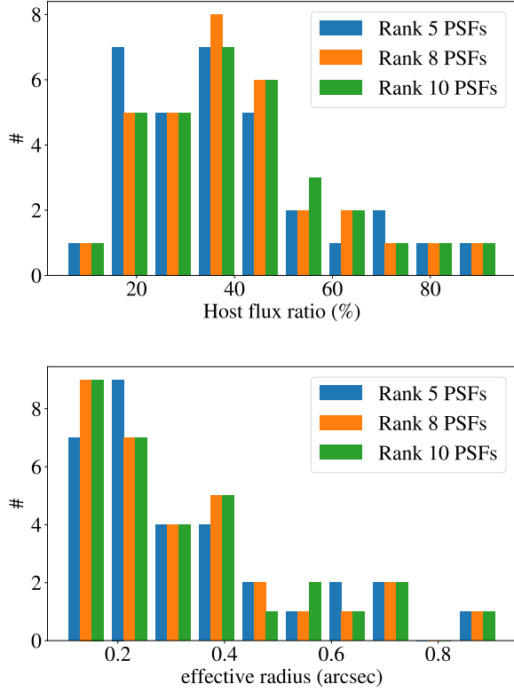
FIG. 3.— Distribution of the host-to-total flux ratio and effective radius when implementing a different number of top-ranked PSFs.
