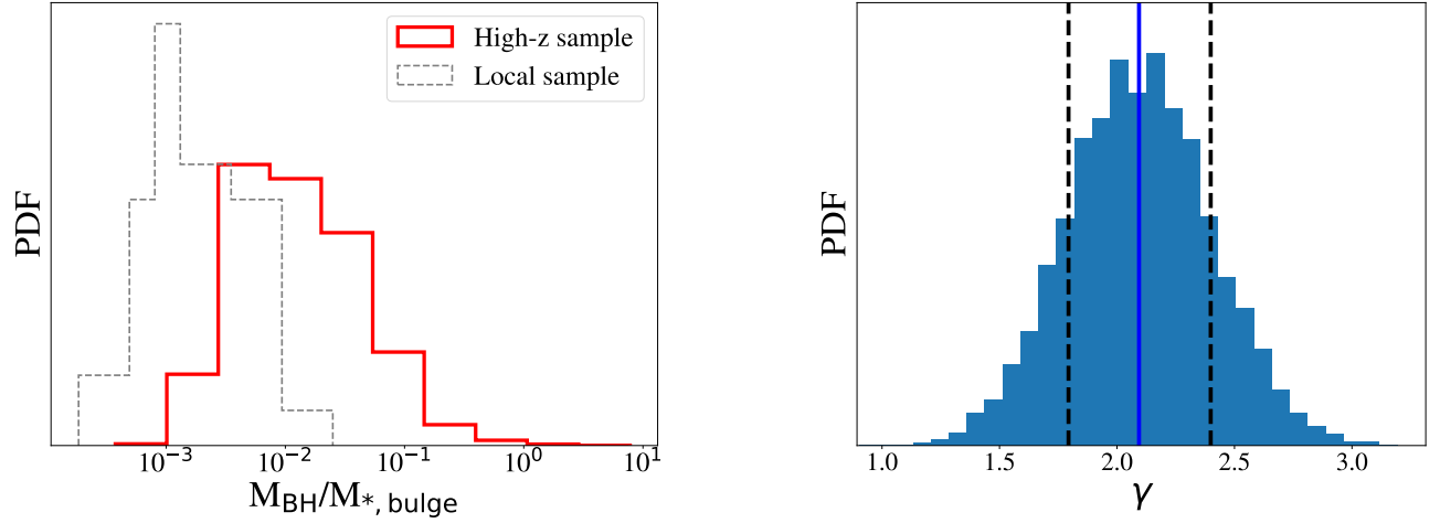
FIG. 12.— Illustration of the distribution from the 10,000 time realizations. Left: \mathcal{M}_{\text{BH}}/M_* distribution for 32 high- z sample, compared to the local one. Right: \gamma distribution, with median value (blue line) and 1\sigma region (dashed line).
