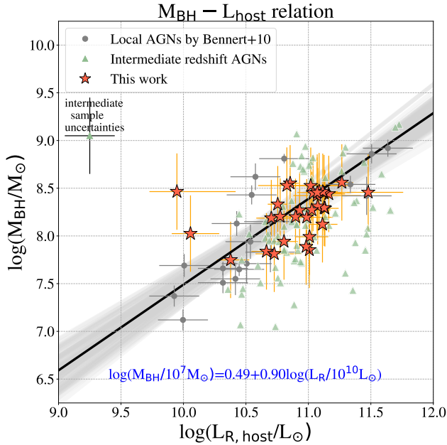
FIG. 6.— The observed black hole mass vs. R-band luminosity relation. The black line and the blue colored equation indicates the best-fit result of the local sample as given in Equation 7, with 1\sigma confidence interval indicated by the gray region. The values for the comparison samples at low and intermediate redshift are listed in Ding et al. (2017b), Table 1 and 2.
