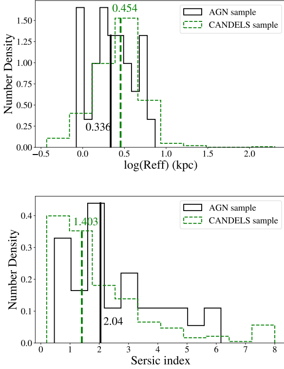
FIG. 4.— The comparison of the histogram of the R_{\text{eff}} (top panel) and Sérsic n_s (bottom panel), with median value indicated. For comparison, we show the distribution of CANDELS galaxies at similar redshifts and stellar masses to our type-1 AGN sample.
