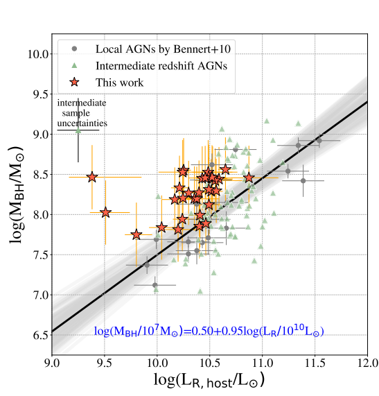
(a) \mathcal{M}_{\text{BH}}\text{-}L_{\text{host}} relation, evolution-corrected
