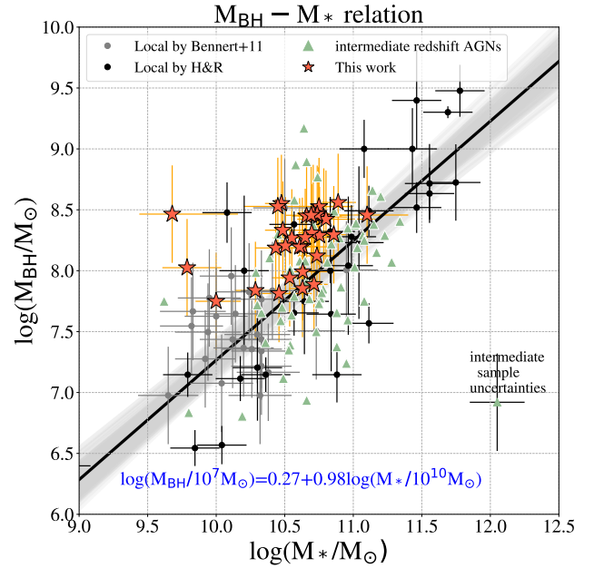
FIG. 7.— Black hole mass vs. stellar mass relation ( \mathcal{M}_{\text{BH}} - M_* ). The best-fit local relation is shown as described in Figure 6.
