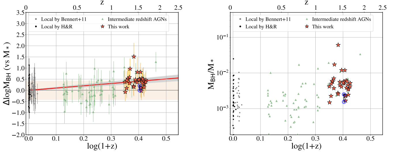
FIG. 8.— Left : Offset in \log(\mathcal{M}_{\text{BH}}) (vs. M_* ) as a function of redshift. The orange band is the intrinsic scatter of local linear relation. The red line and gray band are the best-fit and 1\sigma offset fitting by Equation 9 using our 32 high- z AGNs, with slope value \gamma = 1.03 \pm 0.25 . Right : M_{\text{BH}}/M_* as a function of redshift. In both panels, we use blue open circles to show the expected bias of the median value for \Delta \log \mathcal{M}_{\text{BH}} . We use framework of Schulze & Wisotzki (2011, 2014) to show that even with no evolution selection effects would shift the expectation higher towards the measured values as indicated by the small arrow (Section 2.3.) The measurements of the local and intermediate redshift samples are re-calibrated using self-consistent recipes and listed in Table 7.
