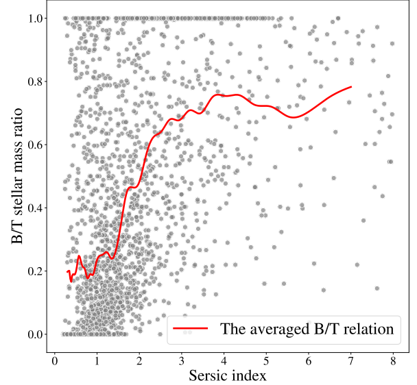
FIG. 11.— Relation between bulge-to-total stellar mass ratio and single-Sérsic index using CANDELS inactive galaxies with \log(M_*/M_\odot) \in [9.0, 11.5] . The red curve is the averaged B/T ratio at different Sérsic index. Note that this curve is only for demonstrating the expected B/T value at different Sérsic index. In this work we adopt the Monte Carlo approach to randomly sample the B/T to account for the scatter.
