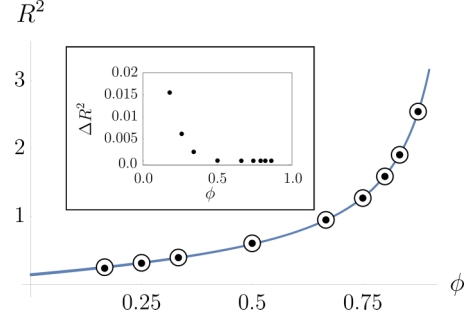
FIG. 2. Range R^2 of the parent Hamiltonian versus magnetic-field strength \phi . Open circles: R_{KM}^2 , corresponding to Eq. (5). Solid dots: R^2 of the most localized parent Hamiltonian. Line is an empirical fit to the solid dots, Eq. (24). Inset: deviation \Delta R^2 = R_{KM}^2 - R^2 .
