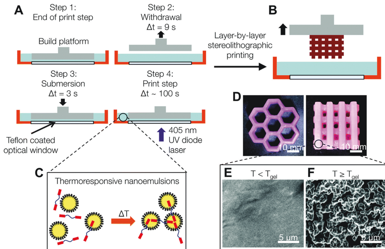
Fig. 22 3D printing of thermo- and photo-responsive PDMS colloids by Doyle et al. Copyright 2017. Reproduced from ref. 11 via Creative Commons License (CC BY-NC 3.0). Published by the Royal Society of Chemistry.
