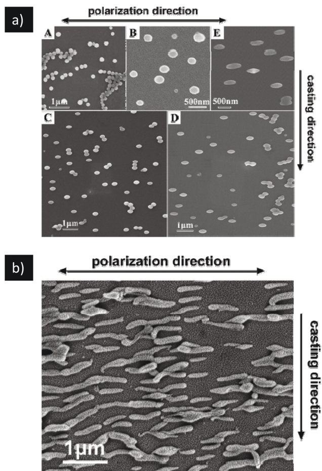
Fig. 14 Li and coworkers investigated the photomechanical deformation of azobenzene containing polymer particles. Irradiation times of 5 (A), 10 (B), 15 (C), 20 (D), and 30 (E) min. Copyright 2006. Reproduced with permission from the American Chemical Society from ref. 183.
