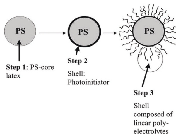
Fig. 3 Guo et al. investigated photo-induced, surface-initiated grafting-from polymerization of polymer “hairs” onto polystyrene latex particles. Copyright 2003. Reproduced with permission from John Wiley & Sons, Ltd from ref. 45.
