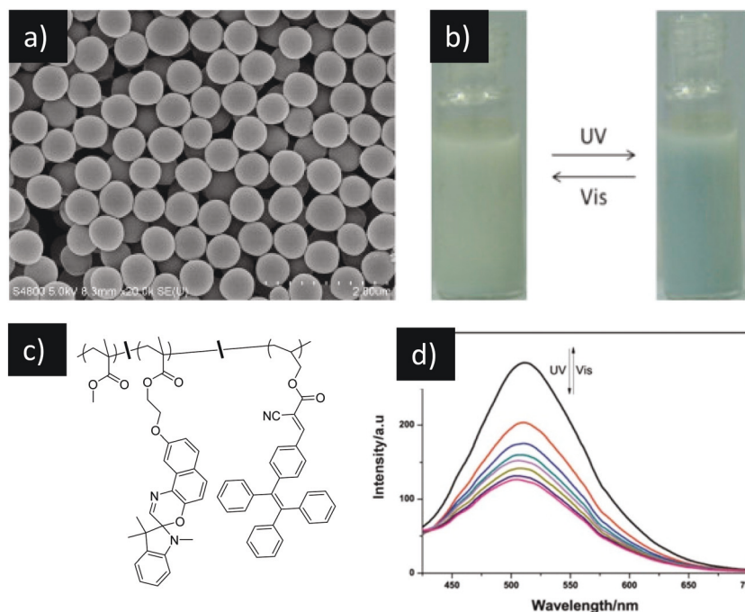
Fig. 11 Li et al. designed latex copolymers containing both AIE luminescent (TPE) and photochromic (SPO) compounds (c) to controllably modulate fluorescence with UV/vis photoswitching (b and d). Copyright 2017. Reproduced with permission from Elsevier from ref. 87.
