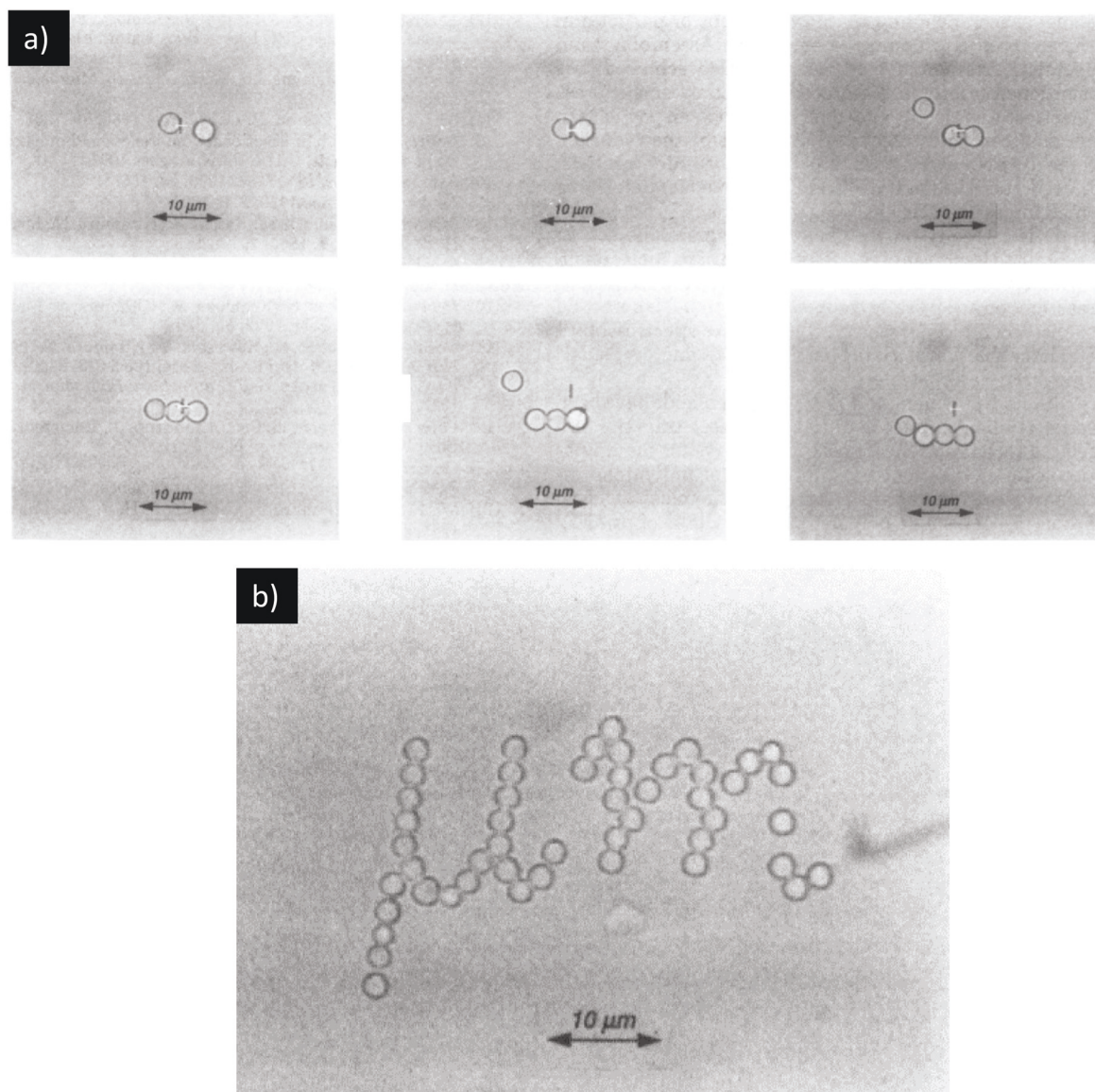
Fig. 20 Misawa et al. utilized light to manipulate and photochemically fixate latex particles via laser trapping and continuous-phase photocrosslinking, respectively. (a) This process enables the forced and permanent assembly of latex particles. (b) illustrates the excellent spatial control for this assembly process to enable fabrication of microscopic patterns. Copyright 1993. Modified and reproduced with permission from the American Chemical Society from ref. 236.
