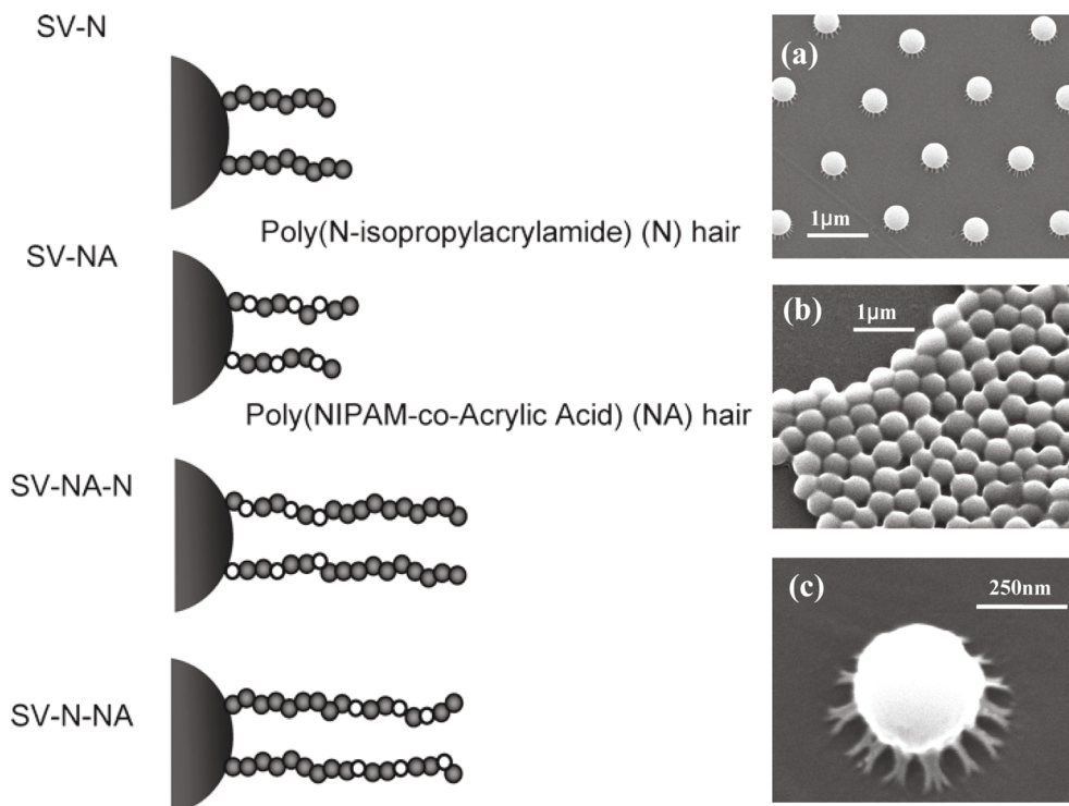
Fig. 4 Tsuji and coworkers designed copolymer functionalized latex particles by photoiniferter controlled radical polymerization from the surface. Copyright 2004. Adapted with permission from the American Chemical Society from ref. 47.
