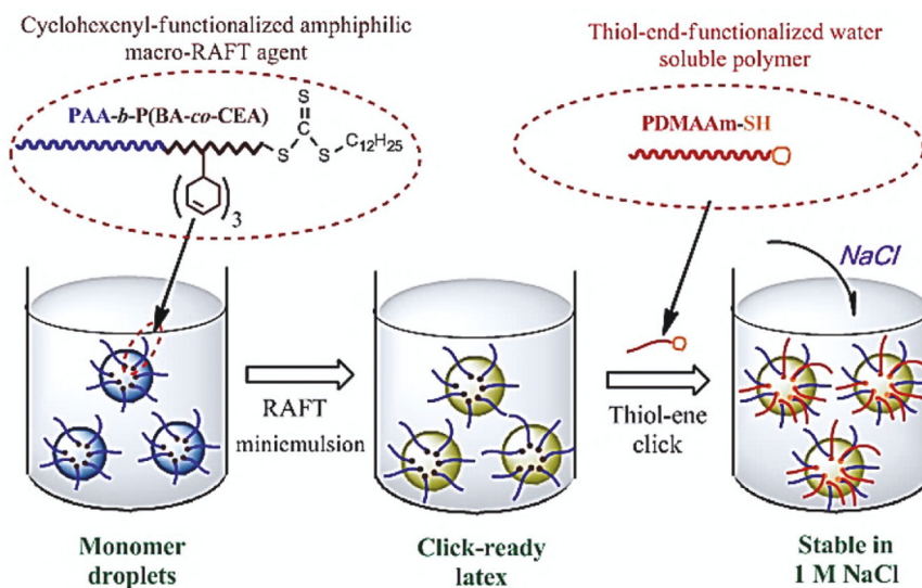
Fig. 5 Yang et al. developed hairy latex particles via thiol-ene “grafting-to” of thiol-functionalized polymer chains to surface-bound alkenes. Copyright 2015. Reproduced with permission from the American Chemical Society from ref. 55.
