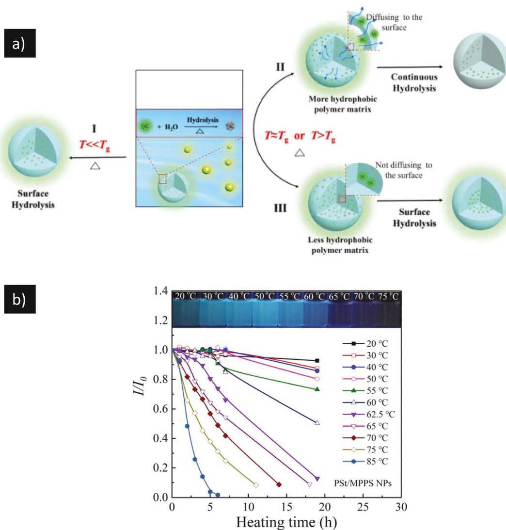
Fig. 12 Liang and coworkers investigated the effects of chain mobility on the protection of water-sensitive AIEgens. (a) Below T_g , AIEgens are kinetically trapped away from the polymer-water interface. However, at and above T_g they can migrate to the surface and hydrolyze. (b) Increased fluorescence loss of MPPS as the temperature approaches the particle T_g (74 °C). Copyright 2019. Reproduced with permission from Elsevier from ref. 90.
