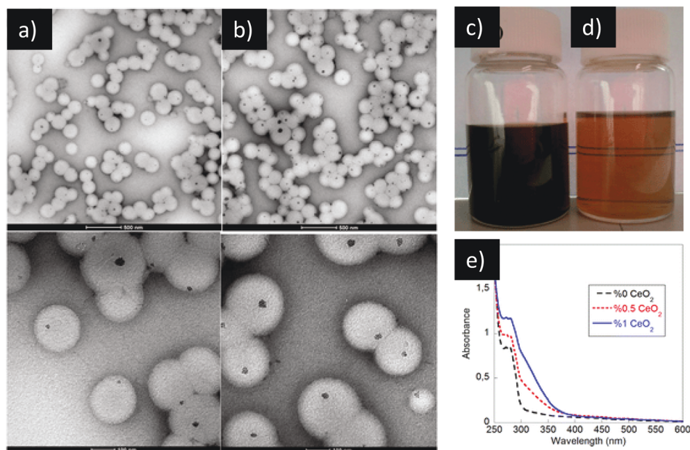
Fig. 6 Aguirre et al. incorporated UV-absorbing CeO 2 nanoparticles into latex via miniemulsion polymerization. (a and b) TEM micrographs of hybrid latexes. (c and d) CeO 2 dispersions in solvent and monomer, respectively. (e) UV absorption of films containing various CeO 2 concentrations. Copyright 2013. Reproduced with permission from the Royal Society of Chemistry from ref. 71.
