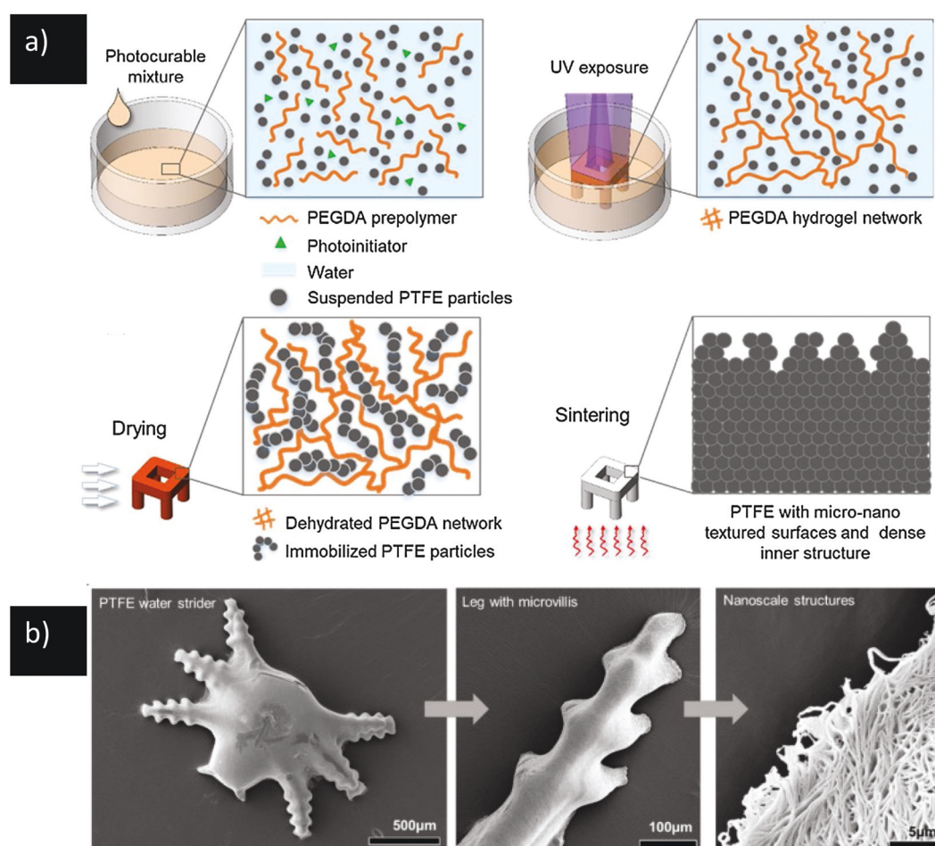
Fig. 23 (a) Zhang et al. printed PTFE colloids via continuous-phase photocrosslinking followed by subsequent thermal degradation of the PEGDA scaffold and sintering of the PTFE particles. (b) 3D printed bionic insect mimics represent an intriguing application for this novel processing capability for PTFE. Copyright 2018. Reproduced with permission from Elsevier from ref. 249.
