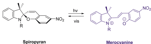
Scheme 1 Photoactivated, reversible photoisomerization of spiropyran to colored, ring-opened merocyanine isomer.
