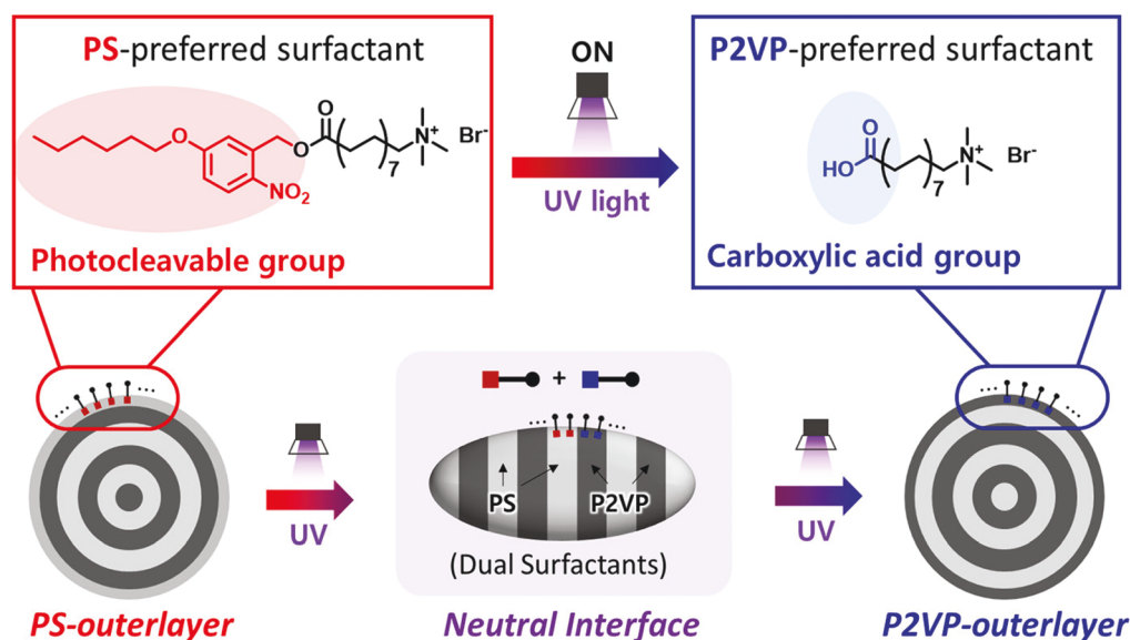
Fig. 17 Lee and coworkers investigated the use of photocleavable surfactants to yield changes in block microphase-separated morphology within latex particles and, as a result, the overall particle shape. Copyright 2019. Reproduced with permission from the American Chemical Society from ref. 193.
