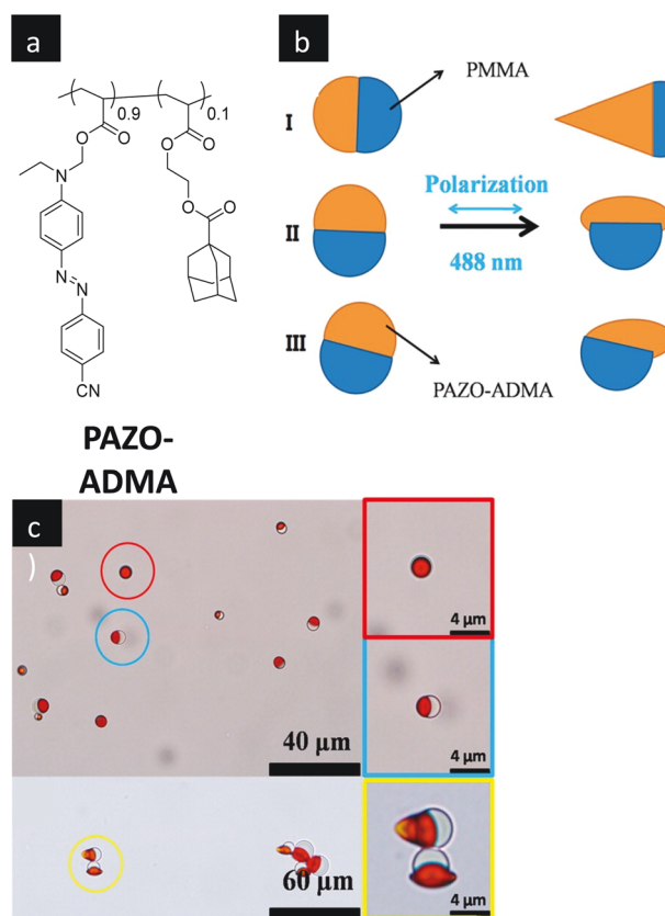
Fig. 15 Zhou and coworkers investigated the photo-deformation of Janus azo-functionalized latex particles. (a) Azo-containing copolymer incorporated into one half of the Janus particles. (b) Effect of orientation on shape of photo-deformed particle (c) optical micrograph of Janus particles before (top) and after (bottom) irradiation. Copyright 2016. Reproduced with permission from the American Chemical Society from ref. 189.
