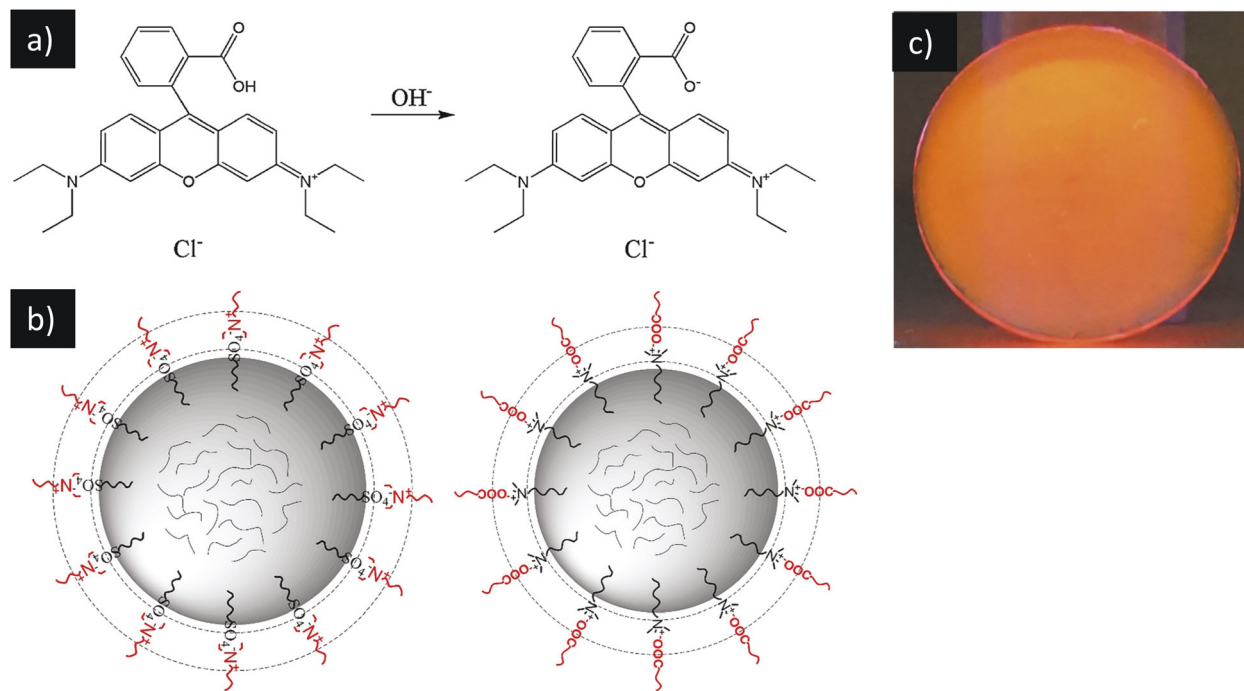
Fig. 9 Li et al. investigated the ionic attachment of rhodamine B (a) to the surface of anionically and cationically charged latex particles (b) to reduce aggregation caused quenching (ACQ) in the resultant films (c). Copyright 2018. Reproduced with permission from Elsevier from ref. 91.
