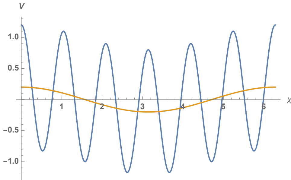
FIG. 2: A sketch of the potential in equation (A1). The blue line is the potential at low temperatures, the orange line is the potential at high temperatures where only the second term in equation (A1) is on. This axion begins in some random minimum in its potential and then ends up in a different one. The vacuum energies of the minima are split by \text{meV}^4 so this can easily raise the negative CC left after relaxation to a positive CC.
