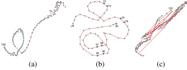
Figure 5: Comparing t-SNE projections using different types of time-varying data sets. (a) ionization, (b) climate, and (c) combustion (CHI). (a) to (c) are for regular, periodic, and turbulent types of data, respectively. Time steps are marked with black dots. In (b), both ends of the periods are highlighted (each period consists of 12 time steps).
