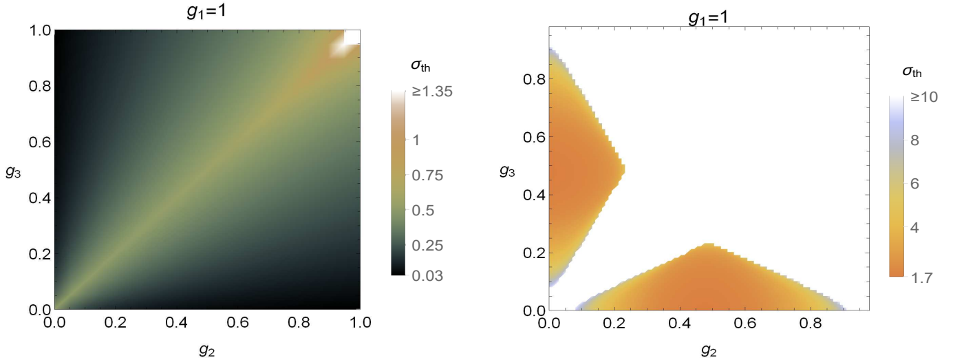
FIG. B2: Left: the pseudothresholds for the n = 3 repetition code. Right: the pseudothresholds for the n = 3 efficient code. In both panels g_{\text{max}} = g_1 is fixed to 1. Without loss of generality, we consider g_1, g_2 \geq 0 .
