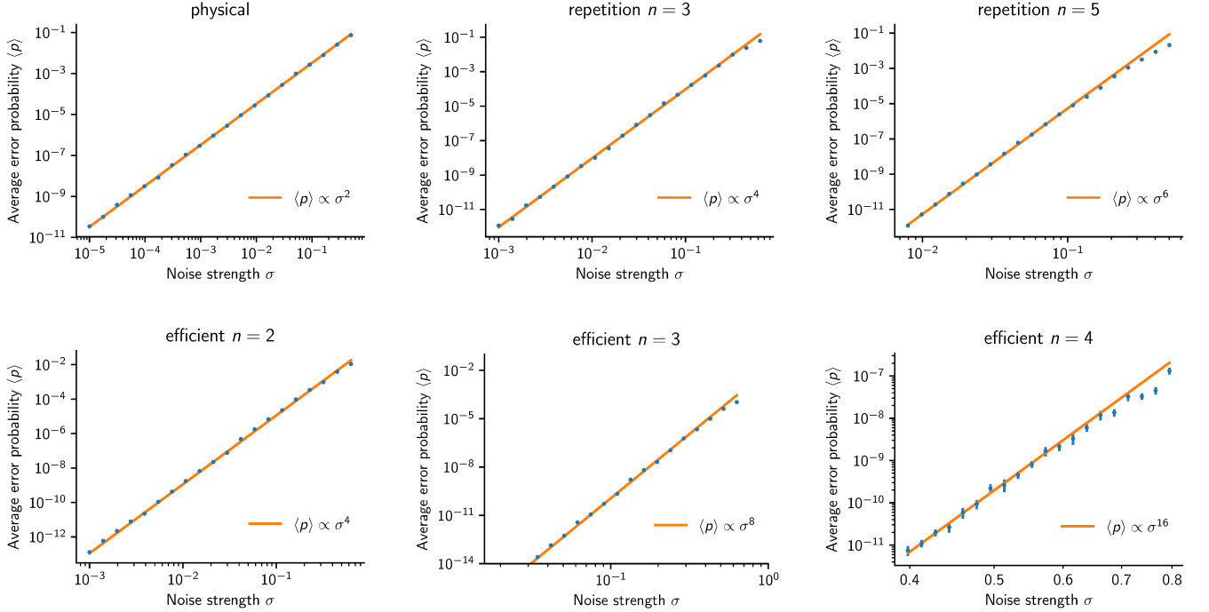
FIG. C2: Further validation of Fig. 1 from the main text, in the ultra-low-noise regime. Each code is shown in a different panel for clarity (along with an unencoded qubit for reference). The blue dots are data points; error bars, when visible, denote standard error of the mean in Monte Carlo averaging. The yellow lines are the corresponding power laws whose slopes serve to guide the eye (their offsets, which were determined through fitting, are not of primary importance here). For clarity, the panels use different ranges of \sigma (unlike the inset of Fig. 1), chosen to be as wide as possible, such that (i) they represent a perturbative regime ( \sigma \lesssim 1 ) where \langle p \rangle is described by a power law, and (ii) they do not produce unmanageably small values of \langle p \rangle prone to significant numerical errors. The hardware-efficient code with n = 5 is not shown because it suppressed noise so strongly that it was difficult to find values of \sigma satisfying both (i) and (ii).
