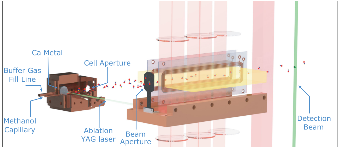
FIG. 2. A rendering of the experimental apparatus. On the far left is the two-stage buffer-gas beam source, depicted in a cut-away view for clarity: 35.5 cm from the exit of the buffer-gas cell, the molecular beam is collimated by a 3 mm square beam aperture, and, 39 cm from the cell, the molecules enter the interaction region where they are addressed with light from the main MO cooling beams in the vertical direction. Copropagating vertically are the (100), (200), and (02 00 ) repumping lasers indicated in red. The (02 20 ) and (01 10 ) repumping light, indicated in yellow, is multipassed in the horizontal direction and extends beyond the MO region. A separate vertically multipassed region containing (100) and (02 00 ) repumping light lies after the magnetic field coils and serves to recover population from excited vibrational states. Finally, the molecules encounter a detection beam of a smaller cross section than the cooling and repumping light, and the resulting laser-induced fluorescence is collected and imaged onto an EMCCD (electron multiplying charge coupled device).
