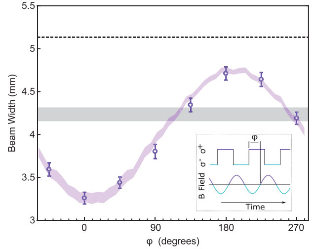
FIG. 4. Molecular beam width as a function of phase offset ( \phi ) between the polarization switching of cooling light and the oscillating magnetic field (see inset). The dashed black line indicates the width of the unperturbed beam, the shaded grey region indicates the measured width and associated error of the Doppler cooled beam without an applied magnetic field, and the shaded purple region indicates Monte Carlo simulation results for the full MO configuration. Clear compression at 0 phase corresponds to the MOT configuration, where the laser polarization provides a spatially confining force. At 180 degrees there is expansion of the beam, corresponding to the anti-MOT configuration. The main cooling light is detuned -7 MHz from resonance while all repumping lasers remain resonant. Error bars represent one standard deviation of the fitted Gaussian beam width.
