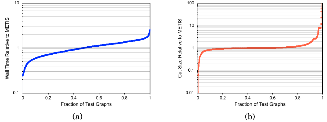
Fig. 4. (a) Overall timing and (b) overall cut quality performance of Mongoose relative to METIS 5. Note the logarithmic vertical scale. Points below the center line represent cases where Mongoose outperforms METIS (relative performance less than one), while points above the center line indicate cases where METIS outperforms Mongoose (relative performance greater than one). In general, Mongoose performs competitively with METIS 5.
