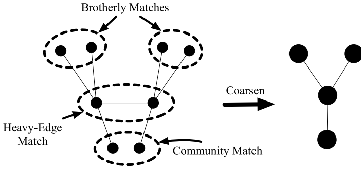
Fig. 3. Community matching.
