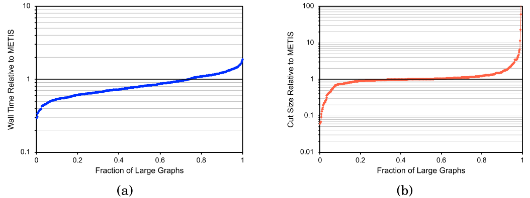
Fig. 5. (a) Timing and (b) cut quality performance profiles [Dolan and Moré 2002] of Mongoose on large graphs (1M+ edges) relative to METIS 5. Note the logarithmic vertical scale. Points below the center line represent cases where Mongoose outperforms METIS (relative performance less than one), while points above the center line indicate cases where METIS outperforms Mongoose (relative performance greater than one).
