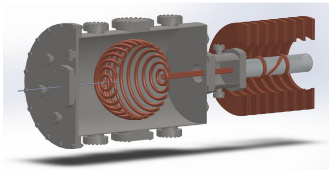
Fig. 2. Cutaway view of the experimental concept showing spherical MPT installed in vacuum chamber. An RF helicon plasma source (at right) produces high density plasma that is channeled by a linear RF multipole stage to the MPT. Details are illustrated in Fig. 3.
