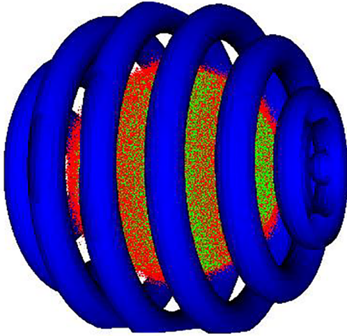
Fig. 1. Particle-in-cell simulation of a 3D MPT with N = 8 , r_0 = 10 cm, loaded with heavy positive particles (green) and light negative particles (red) to simulate quasineutral plasma trapping. (For interpretation of the references to colour in this figure legend, the reader is referred to the web version of this article.)
