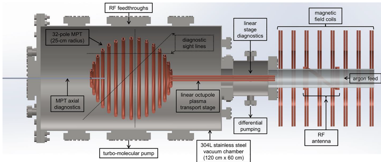
Fig. 3. Side view of cohesive experimental concept comprising helicon plasma source (right), linear RF multipole plasma transport stage (center), and 32-pole multipole plasma trap (left). The main cylindrical vacuum chamber has diameter 60 cm, and is pumped to < 10^{-8} Torr base pressure by a turbo-molecular pump. Several radial and longitudinal ports are available for power feedthroughs or diagnostics, and the MPT may be positioned along the axis accordingly. Differential pumping is utilized in a small module between the helicon source and main chamber to maintain low pressure for the MPT. The magnetic field coils (producing 0–1000 G on-axis) may also be positioned around the small module, and the linear stage may be shortened, such that the linear stage plasma is uniformly magnetized.
