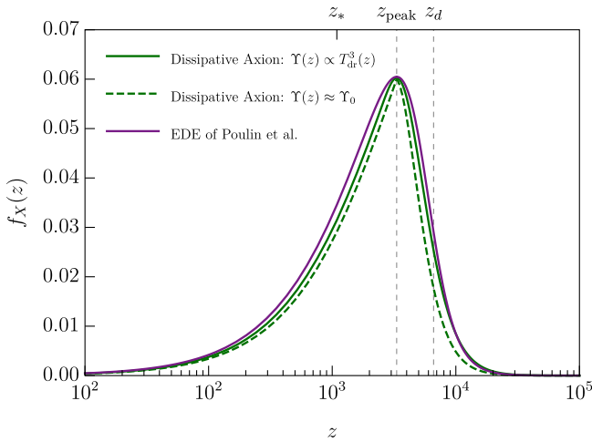
Figure 2. We compare the fractional early dark energy density of the full temperature dependent DA model [ \Upsilon(z) \propto T_{\text{dr}}^3 , solid green] with the semi-analytical approximations in equation (11) and (13), treating the friction as constant [ \Upsilon(z) \approx \Upsilon_0 dashed green] and the EDE fluid approximation of an oscillating scalar field from Poulin et. al. [22] (purple). This plot uses the n = 2 EDE best-fit parameters [ z_c = 5345 , f_{\text{EDE}}(z_c) = 0.044 which corresponds to z_{\text{peak}} = 3322 , f_{\text{EDE}}(z_{\text{peak}}) = 0.060 ] and dissipative axion parameters \frac{\Upsilon(z_{\text{peak}})}{m^2} = 1.3 * 10^{36} \text{ GeV}^{-1} ( \frac{\Upsilon_0}{m^2} = 5.7 * 10^{36} \text{ GeV}^{-1} ), and \frac{1}{2}m^2\phi_0^2 = 0.55 \text{ eV}^4 ( \frac{1}{2}m^2\phi_0^2 = 0.21 \text{ eV}^4 ) for the temperature dependent (independent) DA model.
