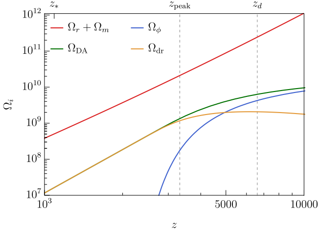
Figure 1. The fractional energy densities \Omega_i = \rho_i/\rho_{\text{crit}} of the different components in the DA and those in a \Lambda CDM universe, where \rho_{\text{crit}} is the critical density today. The total DA contribution (green) is a sum of its sub-components. At early times ( z \gg z_d ), the energy density \Omega_\phi in the scalar field (blue) is roughly constant and the dark radiation component \Omega_{\text{dr}} (yellow) is subdominant. At intermediate times ( z_{\text{peak}} < z < z_d ), the dark radiation \Omega_{\text{dr}} transitions to become dominant as \Omega_\phi drops. Shortly after T_{\text{dr}} reaches a maximum, the total fractional DA energy density peaks at redshift z_{\text{peak}} .
