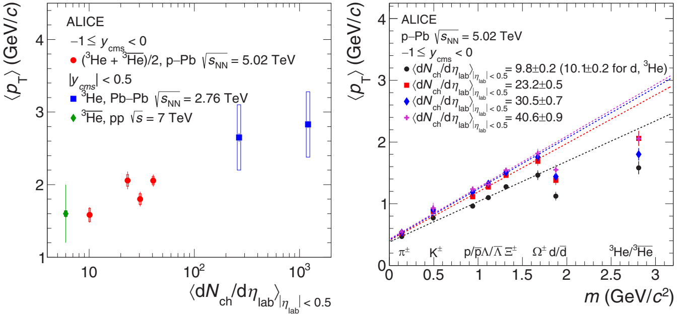
FIG. 6. Left: Mean transverse momentum of (anti-) ^3\text{He} as a function of the mean charged-particle multiplicity density in p -Pb collisions at \sqrt{s_{NN}} = 5.02 TeV. Statistical and systematic uncertainties are indicated by vertical bars and boxes, respectively. The published results from pp [11] and Pb-Pb [12] collisions are shown with diamonds and rectangles, respectively. Right: Mean transverse momentum measured in p -Pb collisions at \sqrt{s_{NN}} = 5.02 TeV as a function of the particle mass is shown for different mean charged-particle multiplicity densities. The linear scaling with the mass found for the results for \pi , K , p , \Lambda [24], \Xi , and \Omega [33] is indicated by dashed lines. The deuteron \langle p_T \rangle is taken from Ref. [34].
