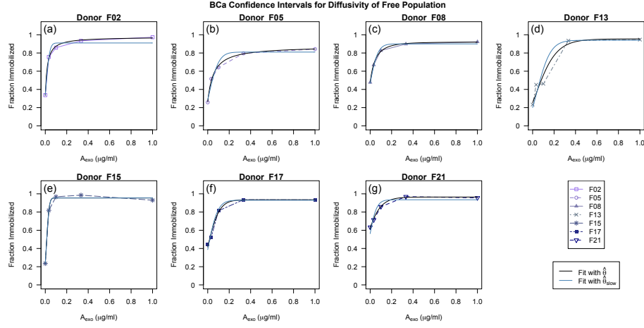
Fig. 14 (a)-(g) For each donor the observed proportion immobilized (dashed lines), proportion immobilized predicted by \tilde{\pi}([A]; \hat{\theta}) , (solid black line), where \hat{\theta} is the numeric estimate for \theta and the proportion immobilized predicted by \tilde{\pi}([A]; \hat{\theta}_{\text{slow}}) (solid blue line), where \hat{\theta}_{\text{slow}} is the numeric estimate restricted to the subspace \Theta_{0.05,5} \cap \Theta_{\text{slow}} . Note in Figure (e) \hat{\theta}_{\text{slow}} = \hat{\theta} .
