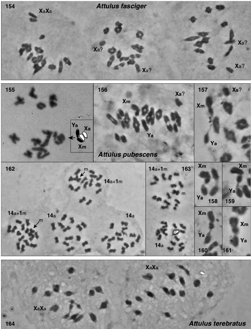
Figures 154–164. Chromosomes of meiosis of Attulus subgenus Sitticus 154 Attulus fasciger , three nuclei, one showing the two Xs together and toward a pole, Canada (43.351N, 79.759W) 155–163 Attulus pubescens , with XaXmYa sex chromosomes, Massachusetts (42.38N, 71.12W) 157–161 XmYa sex chromosomes from other nuclei; the second X is often not paired with them 162, 163 Second division nuclei, all having 14 acrocentrics, and some having in addition a metacentric (m) 164 Attulus terebratus , two nuclei (26a+XaXa0), Novosibirsk Oblast (53.730N, 77.866E).
