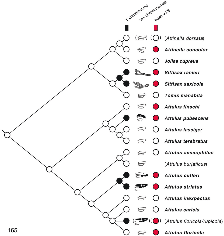
Figure 165. Chromosome evolution in sitticines. Ancestral nodes show the most parsimonious reconstruction of the evolution of Y via X-autosome fusions (black) from the X_1X_20 sex chromosome system (white). Phylogeny from Figure 48 with species added as follows: Attinella concolor is very similar in body and genitalia to A. dorsata ; likewise Sittisax saxicola to S. ranieri ; Attulus caricis position based on their inclusion in the floricola group by Logunov and Kronstedt (1997) and in Sittiflor by Prószyński (2017a). Base chromosome number is directly the number of autosomes if the species has XX0 sex chromosomes, but is interpreted as the number of autosomes +2 if the species has XXY sex chromosomes (apparently derived by a single fusion that would have consumed an autosomal pair), or + 4 if XXXXY (apparently derived by two fusions that would have consumed two pairs). Uncertain scoring is shown by parentheses (see Table 2).
