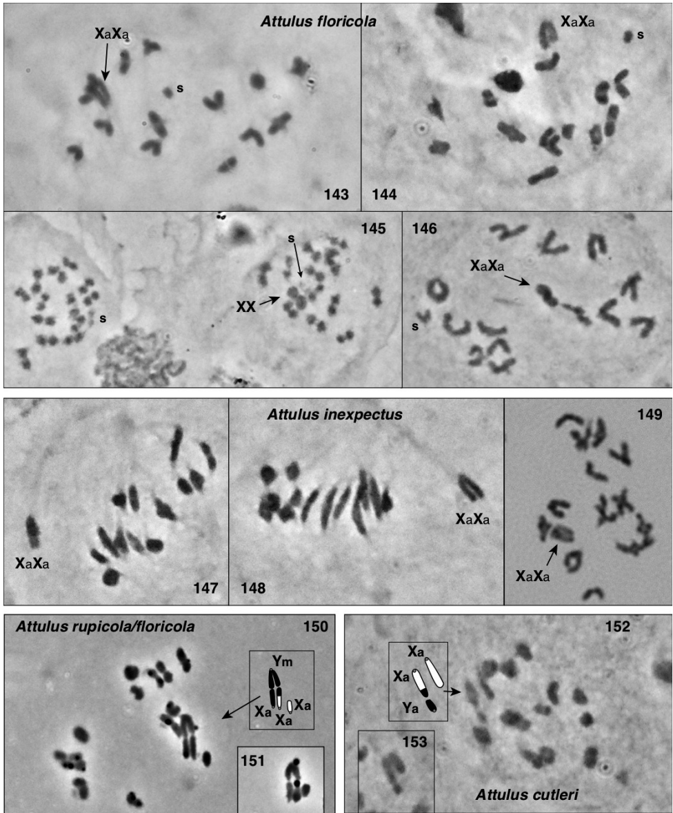
Figures 143–153. Chromosomes of meiosis of Attulus subgenus Attulus , continued 143–146 Attulus floricola , with an extra small bivalent ( s ) to make 28a+XaXa0 , Ontario (44.43, -79.65): 143, 144 first metaphase 145 second division, showing one nucleus with 14 acrocentrics, the other with 14 acrocentrics and the two condensed Xs 147–149 Attulus inexpectus , showing 13 acrocentric bivalents and the sex chromosomes ( 26a+XaXa0 ), Tuva (50.6690, 92.9844) 150, 151 Attulus sp. (ambiguously identified, either A. rupicola or floricola ), tentatively interpreted as having 24a+XaXaXaYm , Switzerland (46.9, 9.2): 151 same, sex chromosomes from another nucleus 152 Attulus cutleri , with 26a+XaXaYa , Canada (68.35, -133.70) 153 same, sex chromosomes from another nucleus
