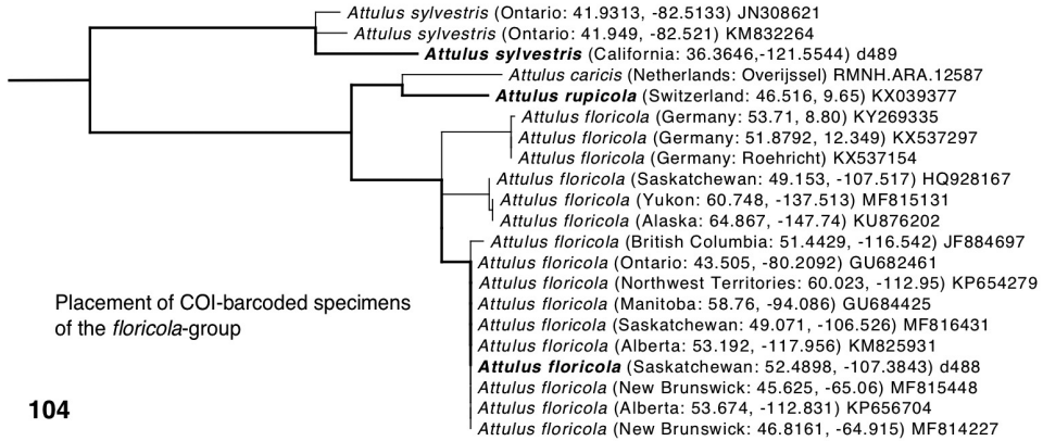
Figure 104. Relationships among Attulus floricola mitochondrial COI sequences in the context of the floricola group. Specimens in bold had their relationships constrained by the UCE phylogeny of Fig. 48; not shown are the relationships outside the floricola group, which are fixed to match the UCE phylogeny. The placement of non-bold specimens on this constrained skeletal tree was inferred by maximum likelihood (RAXML, codon positions as separate partitions).
