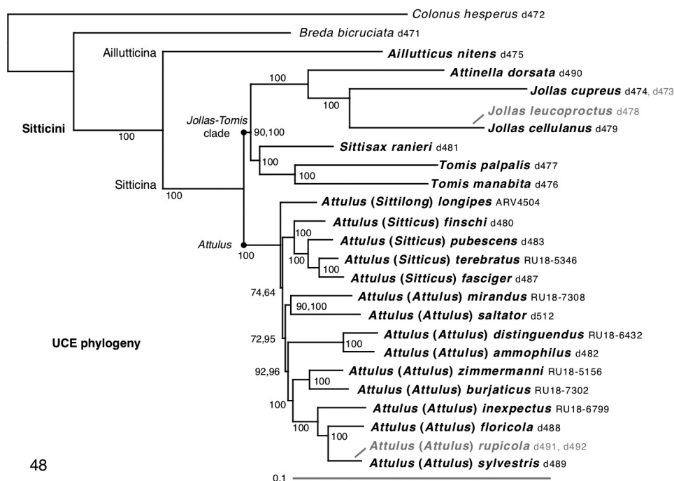
Figure 48. Maximum likelihood phylogeny from 757 concatenated UCE loci (average 113231 base pairs/taxon) analyzed primarily for the 23 Core Taxa in black (IQ-TREE, partitioned by locus). Topology is identical in unpartitioned analyses, with nearly identical branch lengths. Bootstrap percentage values from 1000 replicates shown for each clade. Where two numbers are shown, the first is the bootstrap percentage for the partitioned analysis, the second for the unpartitioned analysis. Where one number is shown, both analyses yielded the same percentage. An analysis of the All Taxa dataset, including the weakly-sequenced taxa in grey, yielded the same topology.
