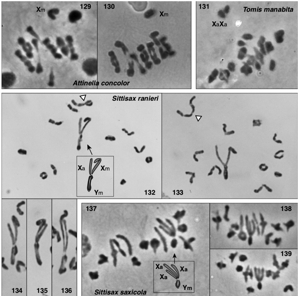
Figures 129–139. Chromosomes of first meiotic division in males of the Jollas-Tomis clade 129, 130 Attinella concolor , with only seven pairs of autosomes, but each two-armed, 14m+X_m0 , Florida (29.63N, 82.37W) 131 Tomis manabita , showing the two Xs off to one pole, and 13 acrocentric bivalents on the metaphase plate, Ecuador (0.9S, 80.5W) 132–136 Sittisax ranieri , whose distinctive X_mX_aY_m appears as a rabbit head with a droopy ear. White triangles show points where two bivalents are apparently linked together 134–136 details of XXY of S. ranieri 137–139 Sittisax saxicola , with sex chromosomes, interpreted tentatively as X_aX_aX_aY_m , appearing as a rabbit head with three ears, Switzerland (46.9N, 9.2E).
