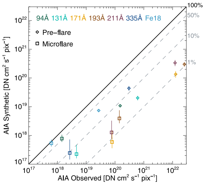
Figure 9. SDO /AIA observed emission vs. the synthetic fluxes derived from the NuSTAR spectral fit (AIA synthetic). The different colors indicate the SDO /AIA channel, and the different symbols represent the pre-flare and microflare times. The solid black line shows where 100% of the observed SDO /AIA would be produced by the material observed by NuSTAR . The gray dashed lines show where the NuSTAR observed emission would be contributing 50%, 10%, or 1% of the emission observed with SDO /AIA.
