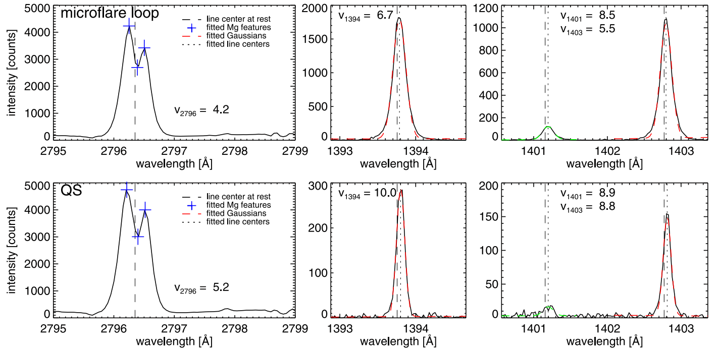
Figure 5. Examples of fits to IRIS line profiles. The top row shows a pixel in the microflare, and the bottom row shows a quiet-Sun pixel. The Doppler velocities are given in \text{km s}^{-1} . For Mg (left column), the feature locations and intensities (blue crosses) are found automatically, while for the other spectral lines, regular Gaussian fits are performed (dashed colored lines).
