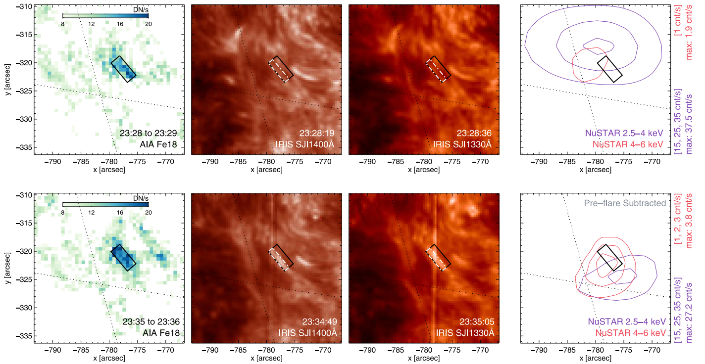
Figure 4. The microflaring region seen in SDO /AIA Fe XVIII, IRIS SJI1400, SJI1330 Å, and contours of the NuSTAR 2.5–4 and 4–6 keV emission (from left to right). The pre-flare time over 23:28–23:29 UT (top row) and the time of the microflare, 23:35–23:36 UT (bottom row), are shown. The solid black rectangle in all panels highlights the location of the SDO /AIA Fe XVIII loop, the dashed-dotted white rectangle in the middle panels indicates the smaller IRIS loop, and both are used to produce the light curves in Figure 2. The same absolute contour levels are used for both times in each NuSTAR energy band, given to the right of the panel with the max value of each image. Note that the NuSTAR contours for the microflaring time (bottom right panel) have the pre-flare image subtracted.
