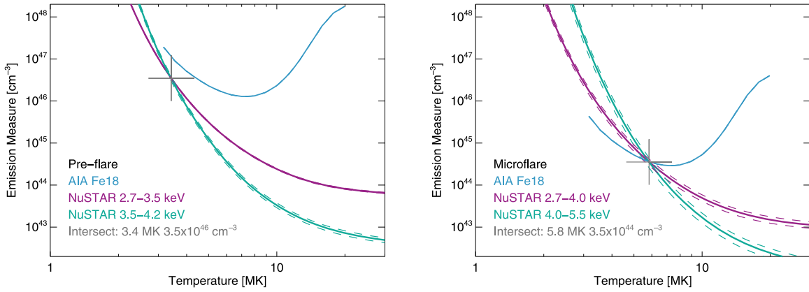
Figure 8. EM loci curves for the pre-flare (left) and microflare excess (right). Shown are the loci curves for two NuSTAR energy ranges, and SDO /AIA Fe XVIII. The dashed lines give the bounds of the uncertainty for each curve. In both panels, the gray cross shows the intersect of the two NuSTAR energy bands, the temperature and emission measure of this point given in the legend.
