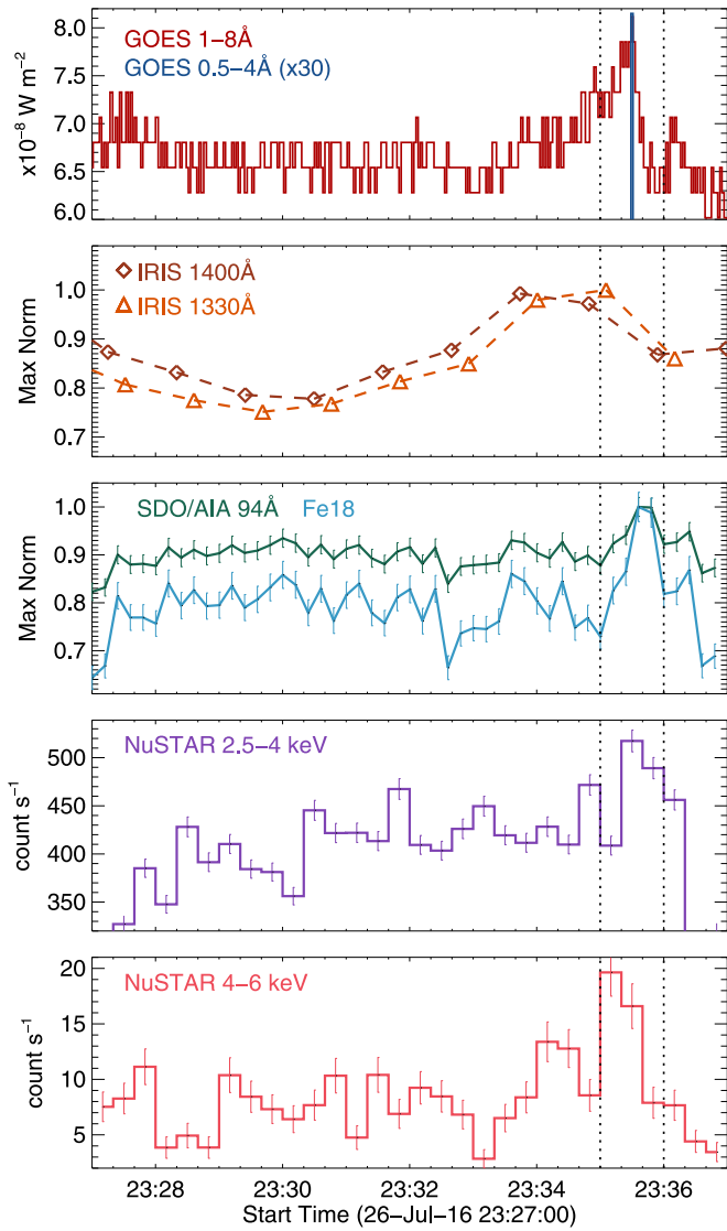
Figure 2. The microflare time profiles from (top to bottom) GOES /XRS 1–8 and 0.5–4 Å, IRIS SJI1400 and SJI1330 Å, SDO /AIA Fe XVIII, NuSTAR 2.5–4 and 4–6 keV. The dotted vertical lines indicate the time of the microflare over 23:35–23:36 UT. Here the GOES light curves (top panel) are from the full-disk emission, whereas the other panels are the box regions highlighted in Figure 4 for SDO /AIA and IRIS and in Figure 3 for NuSTAR .
