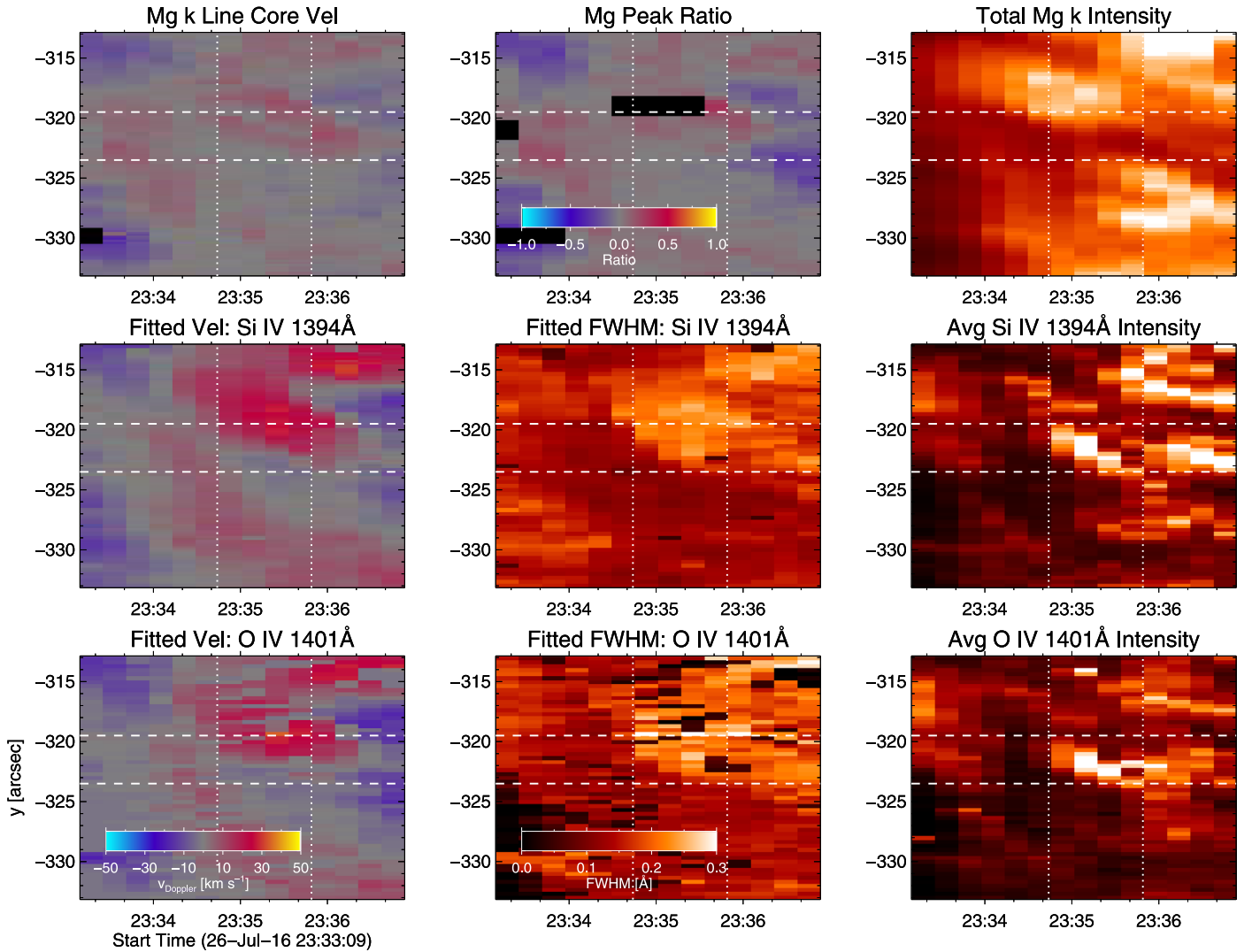
Figure 6. Spectral fit results to the IRIS slit spectrum, using the fitting approach as shown in Figure 5. The top row shows the line core velocity, peak ratio, and total intensity for Mg II. The middle and bottom rows show the fitted velocity, line FWHM, and intensity for Si IV and O IV, respectively. The dotted vertical lines show the time range the slit is over the microflaring loop. The dashed horizontal lines show the vertical extent of the loop.
