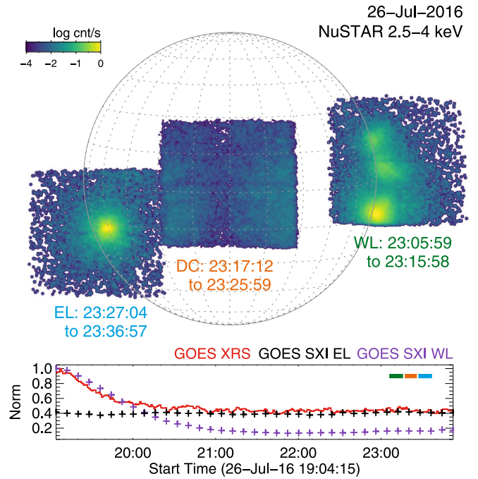
Figure 1. (Top) Full solar disk view of the NuSTAR pointing on 2016 July 26, showing 10 minutes of data from the occulted regions at the west limb (WL) pointing, before the disk center (DC) target, and the region of interest in this paper on the east limb (EL). (Bottom) Time profile of the soft X-rays from the full disk via GOES/XRS 1–8 Å (red line) and from just the WL (purple crosses) and EL (black crosses) regions using the GOES/SXI “Be12a” wavelength.
