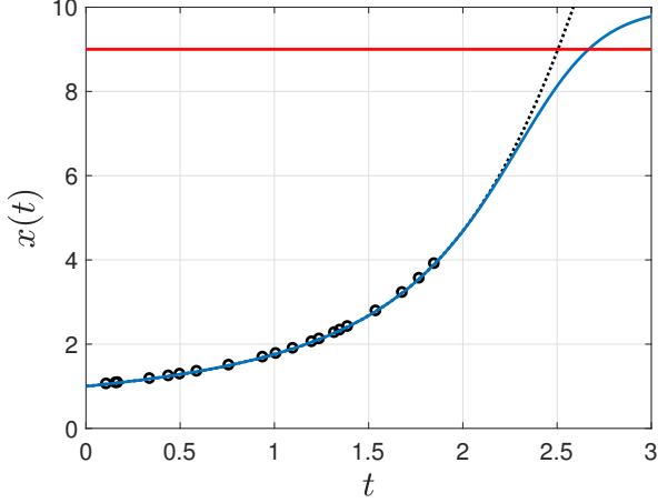
Fig. 1: The boundary of the unsafe set x = 9 (red line), the data points \{x_i\}_{i=1}^{20} (black circles), the piecewise-polynomial approximation of the state X(t) (black dots) and the actual solution of the system (solid blue).
