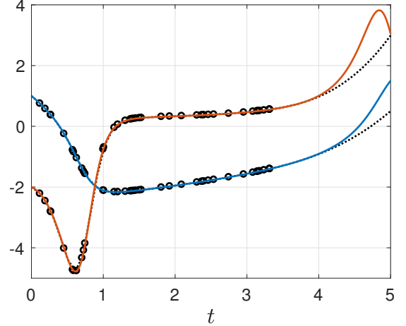
Fig. 3: The data points \{x_i\}_{i=1}^{40} (black circles), the piecewise-polynomial approximation of the state X(t) (black dots) and the actual solution of the system ( x solid blue and y solid red).
