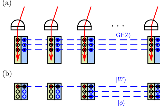
FIG. 4. Interferometry in a multiple-site array. (a) The photon arrival data are decoded using \log_2(M+1) GHZ states. A CZ gate is performed between the memory register at each site and the qubit of the GHZ state. For those registers corresponding to a photon, the phase of the GHZ state is flipped from + to - , which can be read by measuring the qubits of the GHZ state in the X basis. (b) For pairwise readout, acting on a shared W state with local CNOT gates and measuring its qubits in the Z basis projects the network state onto two sites, with probability 1 - 1/N . Otherwise, the W state is transformed into |0, \dots, 0\rangle and measurement can be retried with another W state. Two-side readout proceeds as before, using Bell states for the other registers. After pairwise visibilities are collected, a classical Fourier transform is applied to acquire the desired intensity distribution.
