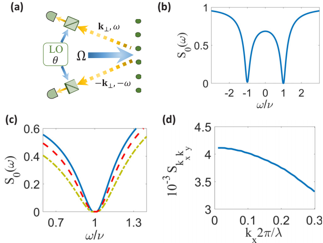
FIG. 5. Quantum squeezing of the reflected field. (a) The correlation between spatiotemporal modes (\pm \mathbf{k}_\perp, \pm \omega) can be observed by homodyne detection at both angles \pm \mathbf{k}_\perp . (b) Squeezing spectrum, Eq. (13), as a function of \omega for fixed \pm \mathbf{k}_\perp = 0 ( S < 1 signifies quantum noise squeezing). The two dips at the corresponding mechanical resonance \pm v_{\mathbf{k}_\perp=0} = \pm v exhibit very strong squeezing, as expected from Eq. (14) [e.g., reaching S \sim 10^{-3} (see panel d) for the specific parameters considered here: a/\lambda = 0.5 , V/E_R = 1500 , trap length 400 nm (yielding \eta \approx 0.12 ), \delta_L - \Delta = -(\gamma + \Gamma)/4 , and uniform illumination with \Omega/\gamma = 0.2 ]. (c) The bandwidth of the squeezing-spectrum dip is determined by the parameter W_{\mathbf{k}_\perp} and can be increased by increasing either a or \Omega [Eqs. (14) and (15)]. This is demonstrated by the red (dashed) curve ( a/\lambda increased to 0.55) and the green (dash-dot) curve ( \Omega/\gamma increased to 0.25), as compared to the blue curve [same as panel (b)]. (d) The dependence of the squeezing on \mathbf{k}_\perp (spatial squeezing) signifies the quantum correlations generated between the spatial modes \pm \mathbf{k}_\perp , reflecting the unique multimode and nonlocal optomechanical response of the array. Here this dependence is plotted as a function of k_x for fixed \omega = v - 12\alpha and k_y = 0 .
