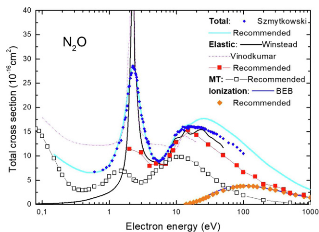
Fig. 10. Comparison between selected experiments, theories and recommended [39] cross sections for \text{N}_2\text{O} . Total experimental [94]; elastic: Schwinger multichannel [90], Q-mol without Born correction [89]; ionization: BEB method [26].
