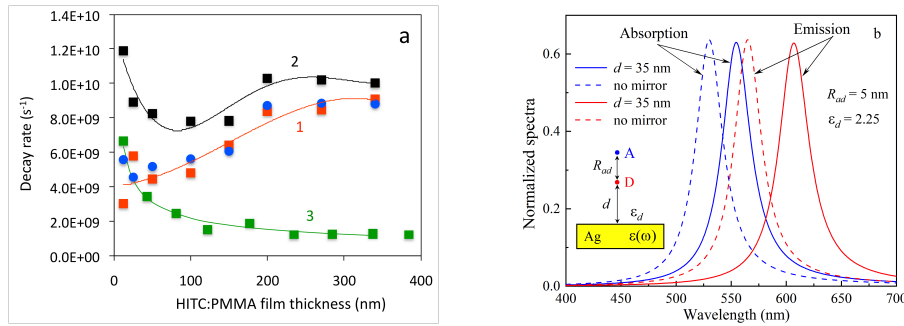
Fig. 1. (a) Trace 1 and red squares: dependence of the emission decay rate on the thickness of the HITC:PMMA film on top of Ag at dye concentration 30 g/l. Trace 2 and black squares: same as above in Fabry-Perot cavities. Trace 3 and green squares: same as above at low dye concentration 3 g/l [5]. Blue circles: Trace 3 subtracted from Trace 2. (b) Calculated normalized absorption and emission spectra in the absence of mirror (dashed lines) and for a vertical donor-acceptor arrangement near the mirror (solid lines)
