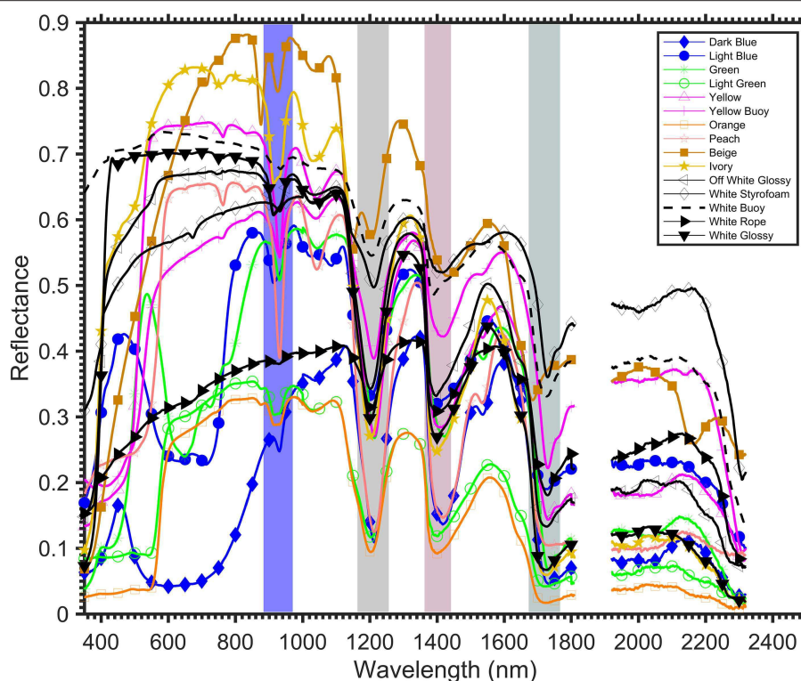
FIGURE 8 | Reflectance of washed ashore macroplastics from beaches along the west coast of the USA reveals spectral absorption features at ~931, 1,215, 1,417, and 1,732 nm (shaded) that are fairly consistent across the variety of plastic objects (adopted from Garaba and Dierssen, 2018) (Garaba holds copyright on this figure).
