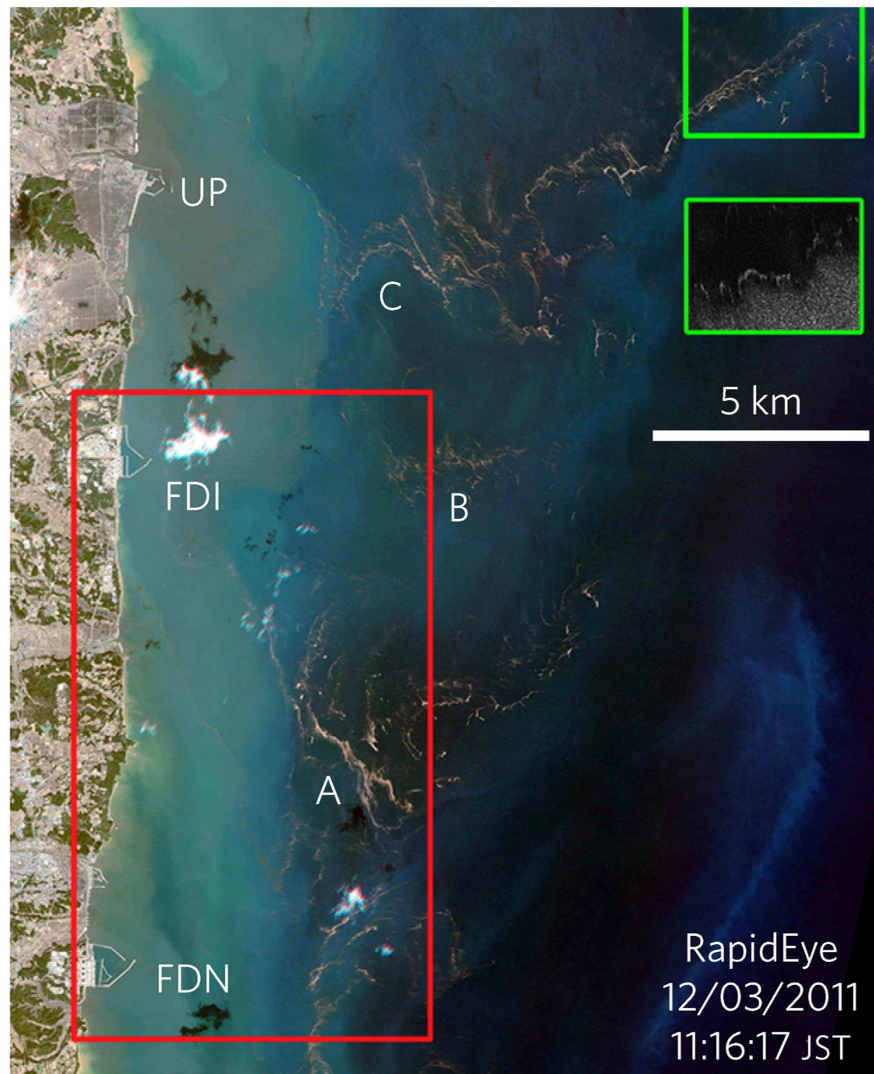
FIGURE 7 | RapidEye image of debris, floating east of Japan 1 day after the March 11, 2011 tsunami showing Ukedo Port (Port), Fukushima Daiichi (FDI) nuclear power station and Fukushima Daiichi (FDN), floating litter A–C visible on 12 March 2011 [Adopted from (Matthews et al., 2017)] (Maximenko has permission from Nature Geosciences to use this figure).
