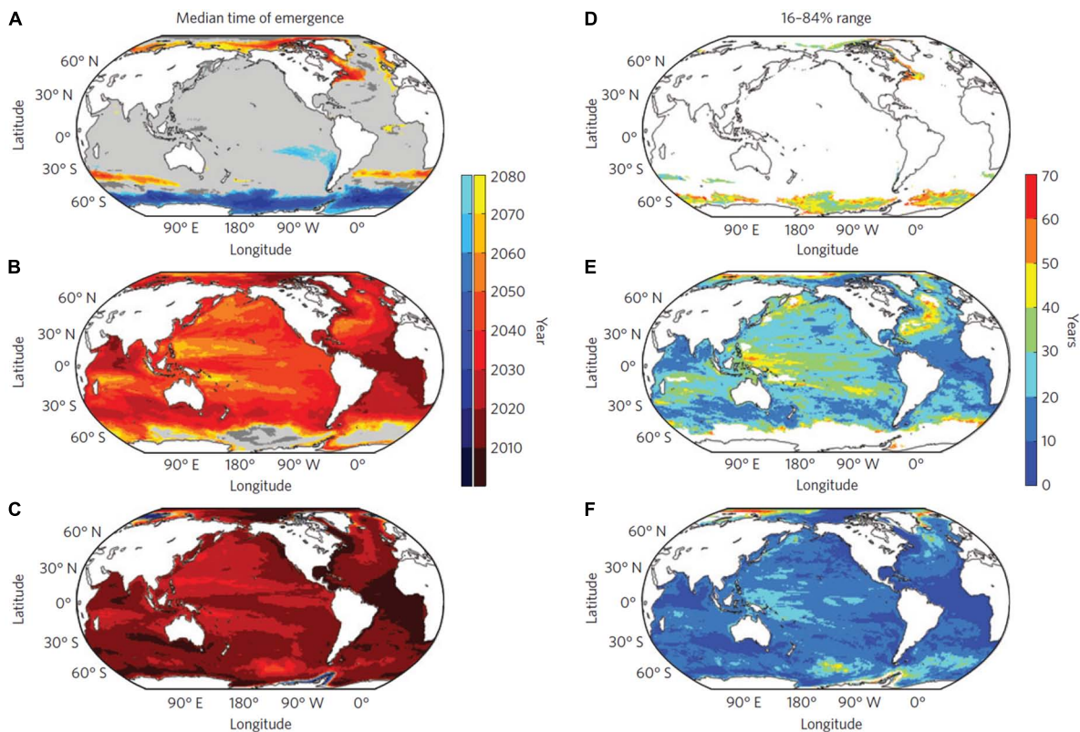
FIGURE 7 | Time after which changes in local sea level are always larger than modeled local sea level variability (ensemble median) under RCP8.5, by year, for: (A) dynamic sea level, (B) dynamic plus global thermosteric sea level, and (C) all contributing components to regional sea level. Gray color means that no signal has yet emerged by 2080 or no agreement between models. The 16–84% uncertainty ranges at regions where at least 84% of the models in the ensemble show signal emergence by 2080 are shown in the right panels (D–F) for the same sea level change projection estimates (A–C) . Adapted with permission from Figure 2 of Lyu et al. (2014).
