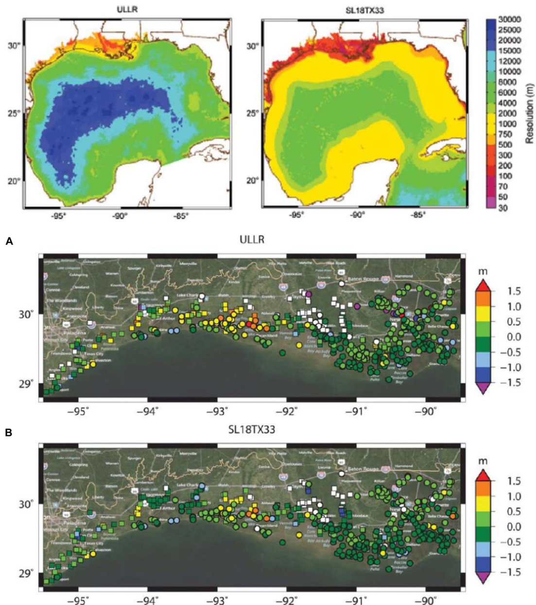
FIGURE 6 | Top panels represent grid resolution in meters of two different model configurations for the Gulf of Mexico (lower resolution labeled ULLR; higher resolution labeled SL18TX33). Locations of Hurricane Ike peak water levels along the northwest Gulf Coast simulated by (A) ULLR and (B) SL18TX33 (circles), and measured by hydrographs (squares). The points are color-coded to show the errors between measured and modeled peak water levels. Green points indicate matches within 0.5 m and white points indicate locations that were never wetted by the model. Adapted with permission from Kerr et al. (2013).
