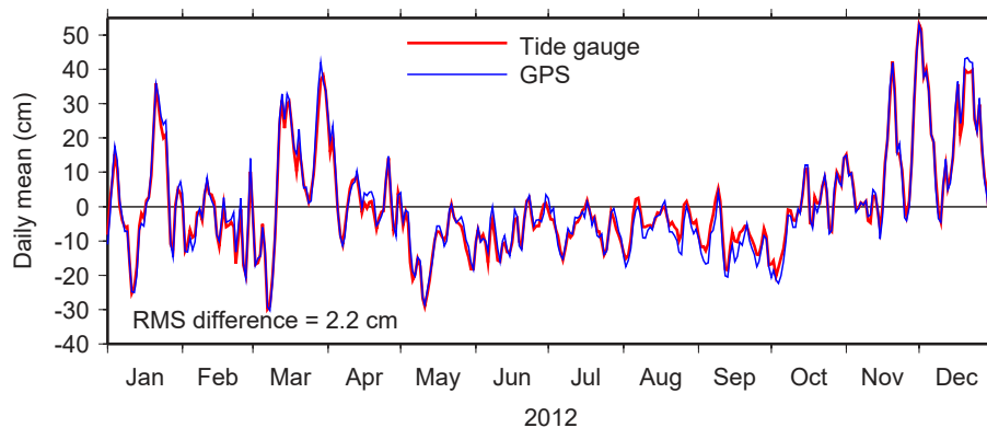
FIGURE 4 | Daily mean sea level during 2012 at Friday Harbor, Washington, United States, in the Strait of Juan de Fuca. Red line is daily means deduced from the Friday Harbor tide gauge, operated by NOAA; blue line is daily means determined by analysis of GPS reflected signals at station SC02, sited 300 m from the tide gauge. Adapted from Larson et al. (2017), who give further comparisons over a 10-year period, including comparisons of tidal constants.
