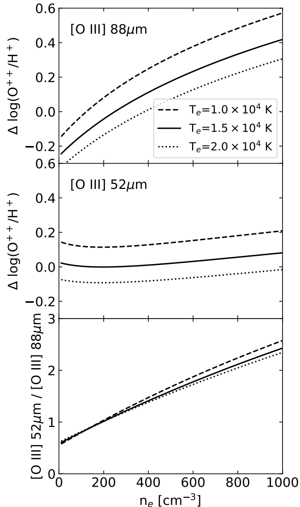
FIG. 2.— Illustration of how assumed density and temperature values affect the derived metallicity. The top panel shows how derived \text{O}^{++} abundance varies relative to the fiducial values (Section 2) at fixed [\text{O III}] 88\mu\text{m} flux. A strong dependence on n_e is apparent due to suppression of [\text{O III}] 88\mu\text{m} emission by collisional de-excitation. In contrast, the middle panel shows that [\text{O III}] 52\mu\text{m} -based abundance is nearly independent of density for n_e \lesssim 1000 \text{ cm}^{-3} , with only modest temperature dependence. [\text{O III}] 52\mu\text{m} is therefore a promising metallicity diagnostic for future work. The bottom panel demonstrates how the [\text{O III}] doublet ratio is a robust density diagnostic (e.g., Palay et al. 2012), with [\text{O III}] 52\mu\text{m} becoming the stronger line at n_e > 200 \text{ cm}^{-3} .
