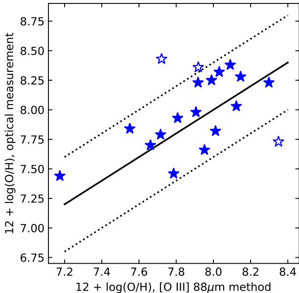
FIG. 1.— Comparison of 12 + \log(\text{O}/\text{H}) determined from [\text{O III}] 88\mu\text{m} and SFR, compared to measurements based on standard optical emission line methods (using [\text{O III}]\lambda 4363 as a T_e diagnostic). Blue stars show all galaxies with suitable [\text{O III}] 88\mu\text{m} measurements from Herschel taken as part of the Dwarf Galaxy Survey (DGS). The solid black line shows the one-to-one relation, with dashed lines at \pm 0.4 dex (corresponding to 2\sigma scatter of the solid symbols), demonstrating reasonably good agreement. The three galaxies which differ by > 0.4 dex (open symbols) can all be reconciled with direct measurements as discussed in the text.
