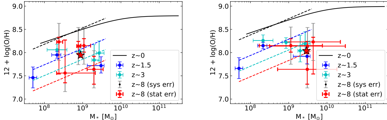
FIG. 3.— Mass-metallicity relation of z > 7 galaxies, compared with z \simeq 1.5\text{--}3.5 galaxies with [\text{O III}]\lambda 4363 -based measurements listed in Table 3, and the z \simeq 0 relation from stacked spectra (black line; Curti et al. 2020). Theoretical simulation-based results from Ma et al. (2016) are shown as dashed lines with the same redshift color-coding ( z = 0, 1.5, 3 , and 8).
