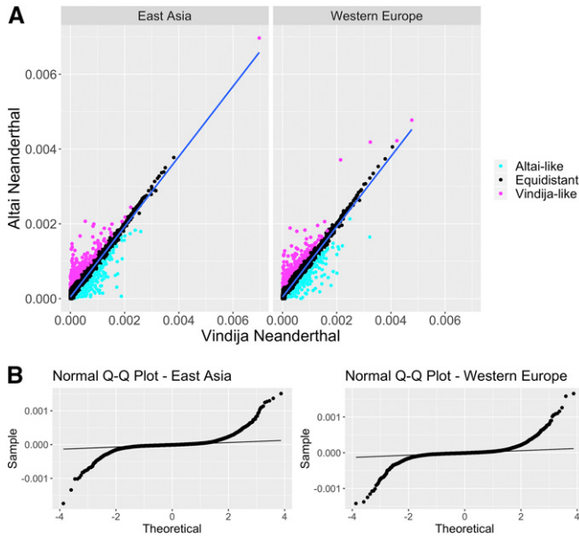
Figure 2 Pairwise nucleotide distances between putatively introgressed haplotypes and Neanderthal genomes. (A) Average pairwise nucleotide differences ( \pi ) between the Neanderthal-introgressed haplotypes detected for 200 genomes from each of East Asian and European populations included in the 1000 Genomes Project data set (Phase I) and the Vindija (x-axis) and Altai Neanderthal genomes (y-axis). The blue lines show the linear regression of the form Y = 4.3 \times 10^{-5} + 9.4 \times 10^{-1} \times X + \epsilon , where \pi between introgressed haplotypes and the Vindija genome ( X ) is used to predict \pi between introgressed haplotypes and the Altai Neanderthal genome ( Y ), and \epsilon is residuals. Residuals of these linear regressions are used to detect Vindija-like and Altai-like haplotypes. Haplotypes with residuals below the 0.025 quantile value of the empirical distribution are considered as Altai-like and shown in cyan. Haplotypes with residuals above the 0.975 quantile value of the empirical distribution are considered as Vindija-like and shown in magenta. (B) Normal quantile-quantile (Q-Q) plots for the residuals of the linear regressions between the variables on the x- and y-axes of A.
