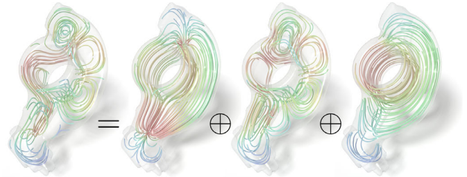
Fig. 4. Helmholtz-Hodge decomposition. On this example, a tangential field is decomposed into the orthogonal sum of a tangential gradient field, a tangential curl field, and a tangential harmonic field.
