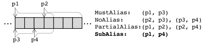
Figure 4. Difference between MustAlias, NoAlias, PartialAlias, and SubAlias. Arrows represent the pointed memory addresses, and dashed lines denote access sizes. Only the most precise result is presented. Analysis may return MayAlias when it cannot infer any other relation.
