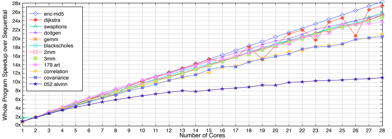
Figure 5. Perspective’s Fully Automatic Whole Program Speedup over Sequential Execution
