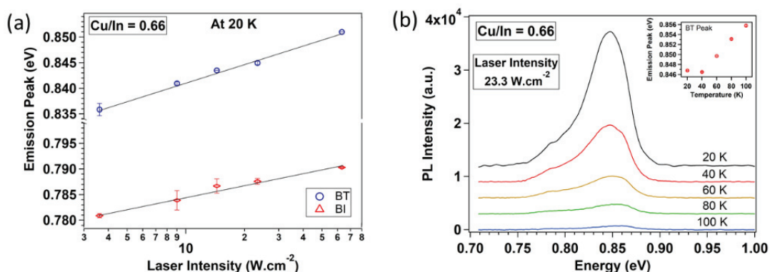
Figure 2. (a) Peak emission vs. laser intensity at 20 K and (b) temperature dependence of PL intensity of CuInSe 2 film with Cu/In = 0.66.
