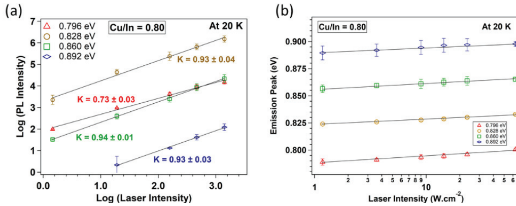
Figure 4. (a) Power law dependence for observed peaks and (b) emission peak vs. laser intensity in \text{CuInSe}_2 film with \text{Cu/In} = 0.80 .
