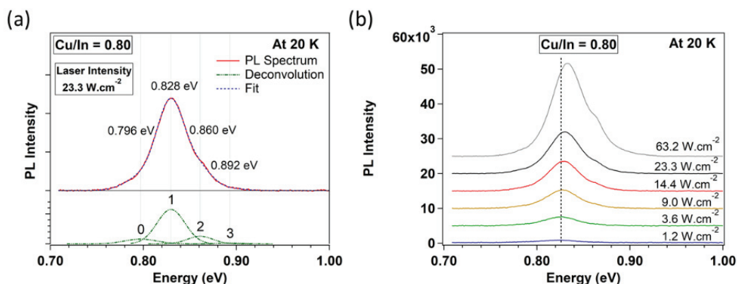
Figure 3. (a) PL spectrum along with multi-gaussian fits and (b) laser excitation dependent PL of CuInSe 2 films with Cu/In = 0.80.
