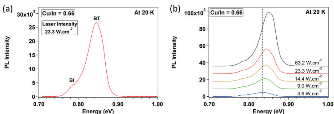
Figure 1. PL spectra of CuInSe 2 film with Cu/In = 0.66 taken at 20 K (a) showing BT and BI band (b) for various intensities of laser.
